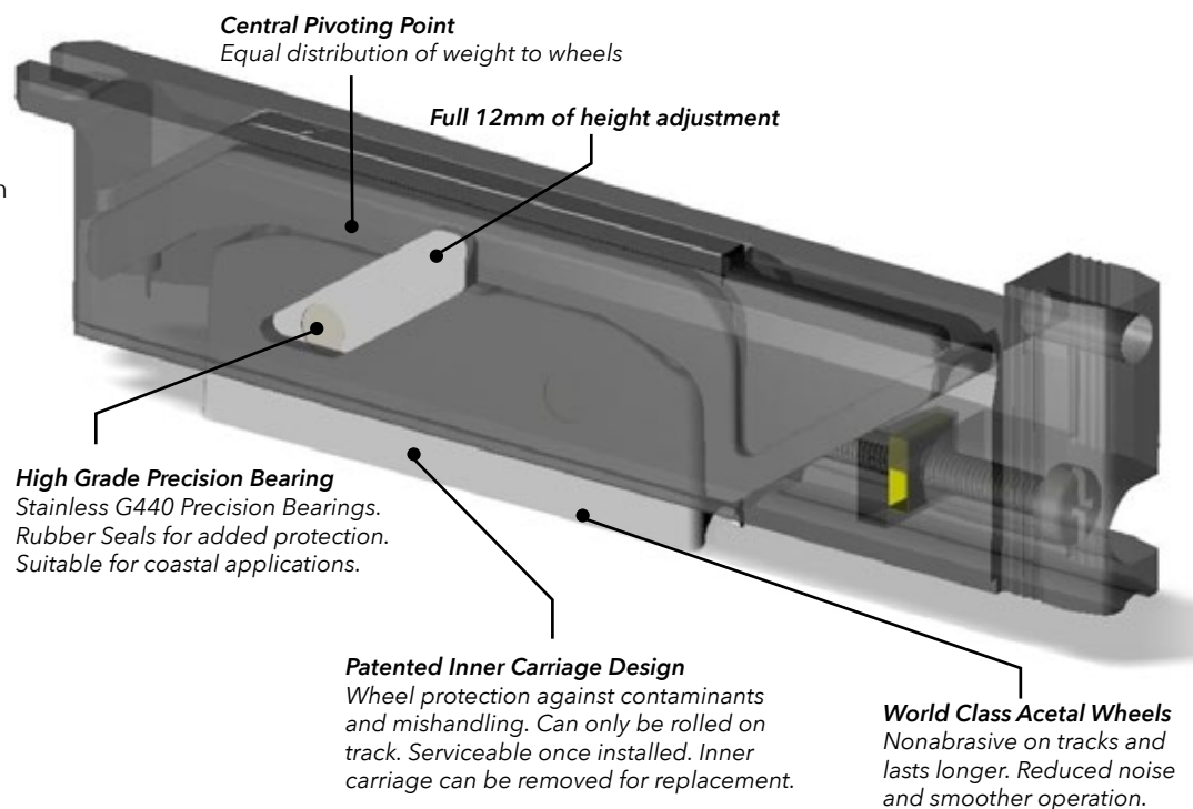
SINGLE WHEEL SS BEARING ROLLER (50KG)
