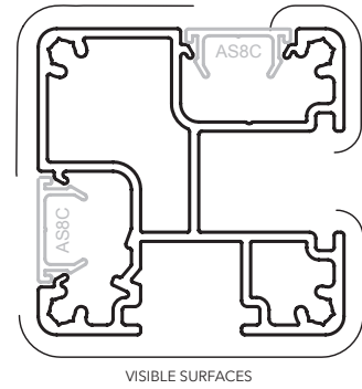
FP58 POST INFILL 1620113
