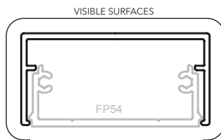
FP54 TOP RAIL BASE 1629557
