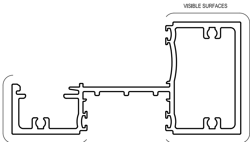
ECO225 100mm DOUBLE GLAZED HOLLOW TRANSOM
