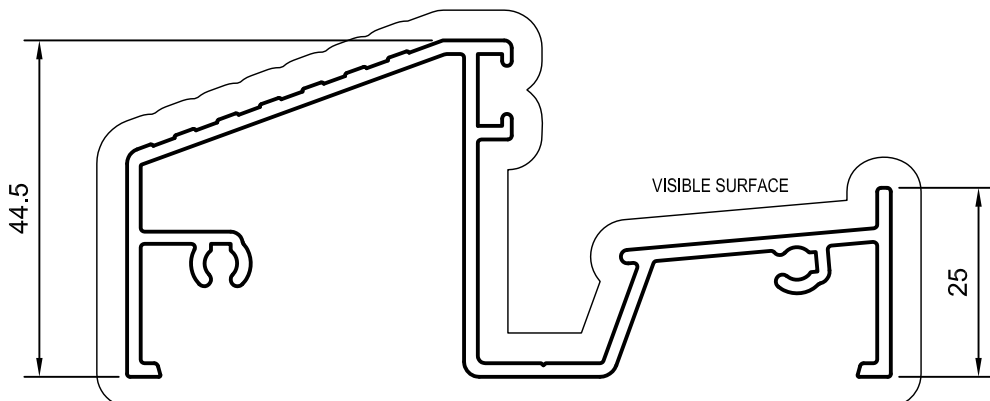
AS2371 HINGED DOOR INWARD OPENING (NEW)
