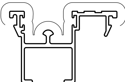
AD788 SCREEN SILL ADAPTOR
