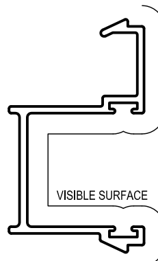
AD789 SCREEN JAMB ADAPTOR
