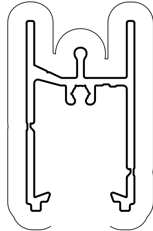
AD761 SCREEN DOOR ADAPTOR SILL
