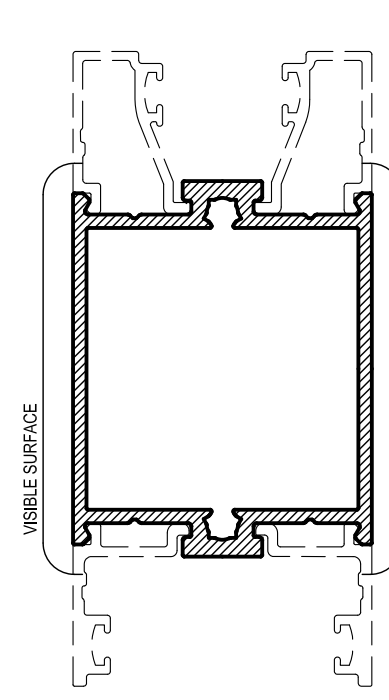
AFD15 40 x 85 MID RAIL Mass. 0,963 Kg/m Anod. Per. 212 Paint Per. 100
