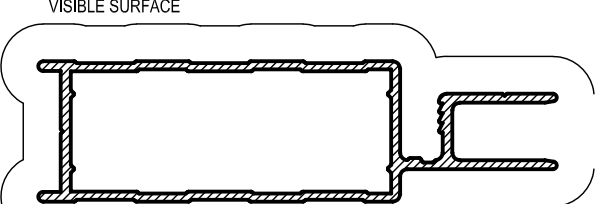
SD9 DOOR FRAME Mass. 0,559 Kg/m Anod. Per. 227 Paint Per. 192
