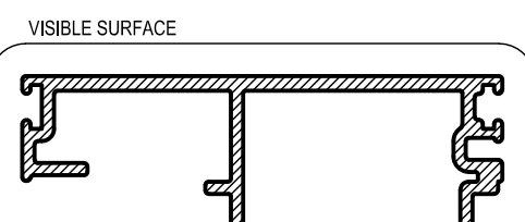
AF316 40mm DG CLIP IN DOOR ADAPTOR Mass. 0,638 Kg/m Anod. Per. 391 Paint Per. 100
