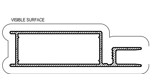
SD2 DOOR FRAME Mass. 0,591 Kg/m Anod. Per. 228 Paint Per. 194
