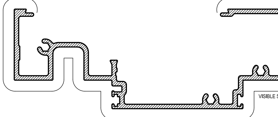
AF15 POCKET INFILL Mass. 0,172 Kg/m Anod. Per. 100 Paint Per. 100
