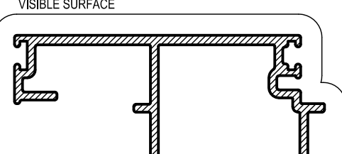
AF317 45mm DG CLIP IN DOOR ADAPTOR Mass. 0,616 Kg/m Anod. Per. 286 Paint Per. 100
