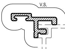
MFA29 MEETING STILE ADAPTOR Mass. 0,215 Kg/m Anod. Per. 100 Paint Per. 100
