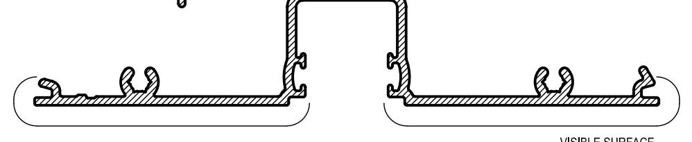
AF213 GLAZING ADAPTOR Mass. 0,930 Kg/m Anod. Per. 408 Paint Per. 102 Ixx = 383,34 x 10 3 mm 4 Iyy = 16,52 x 10 3 mm 4
