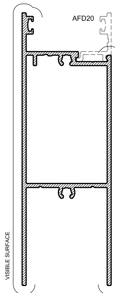
AFD20 40mm DG DEEP RAIL Mass. 1,595 Kg/m Anod. Per. 452 Paint Per. 237
