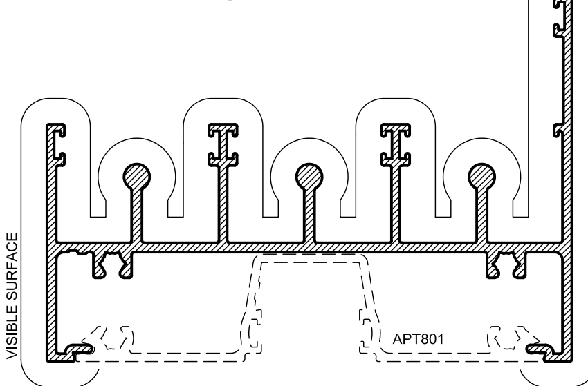
APT94S 101.6mm HIGH PERFORMANCE SILL (PART SLOTTED)
