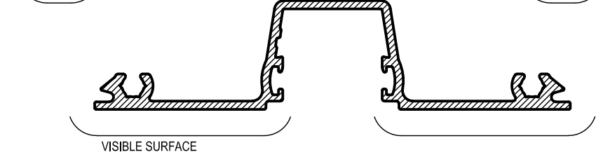
APT801 GLAZING ADAPTOR (ME POCKET)
