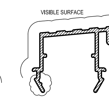
APT33 INTERNAL MID THRESHOLD
