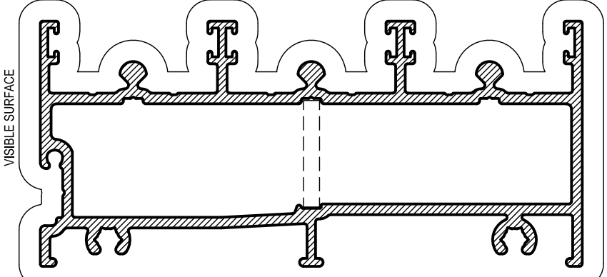
APT64S HOLLOW SILL (INCL TRACK)
