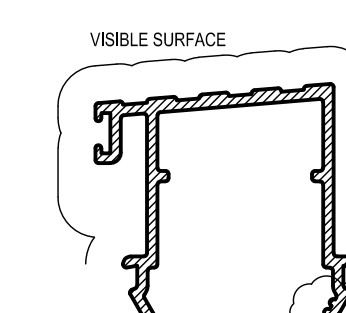
APT30 EXTRA HIGH THRESHOLD
