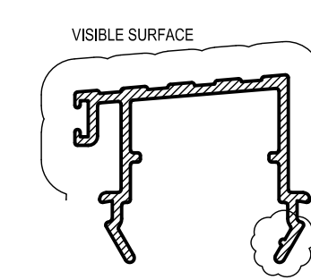
APT6 MID THRESHOLD
