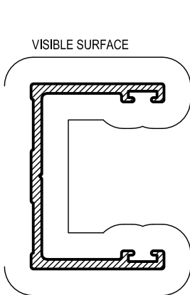
APT42 PLANT ON JAMB ADAPTOR Mass. 0,412 Kg/m Anod Per. 187 Paint Per. 152
