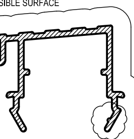
APT6 MID THRESHOLD Mass. 0,412 Kg/m Anod Per. 209 Paint Per. 100
