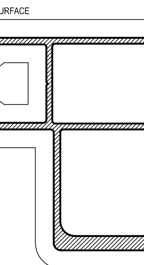
APT31 SG OXO MEDIUM STILE Mass. 1,692 Kg/m Anod Per. 389 Paint Per. 306 Ixx = 279.37 x 10 3 mm 4 Iyy = 246.36 x 10 3 mm 4
