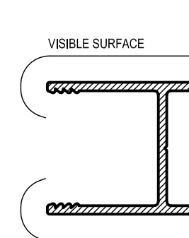
APT19 DG LOCK STILE Mass. 0,693 Kg/m Anod Per. 212 Paint Per. 143
