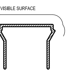
APT5 TRACK INFILL Mass. 0,252 Kg/m Anod Per. 148 Paint Per. 100
