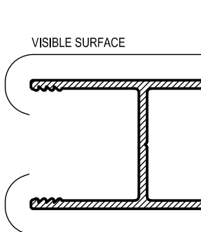
APT23 DG OXO STILE Mass. 0,736 Kg/m Anod Per. 233 Paint Per. 166 Ixx = 25.72 x 10 3 mm 4 Iyy = 73.05 x 10 3 mm 4
