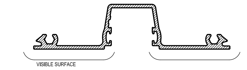
APT801 GLAZING ADAPTOR (ME POCKET) Mass. 0,713 Kg/m Anod Per. 315 Paint Per. 100
