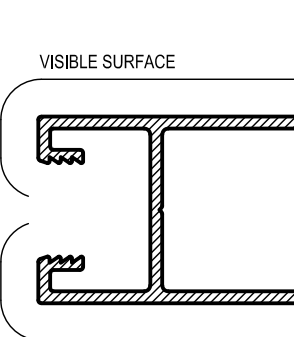
APT13 SG OXO STILE Mass. 0,805 Kg/m Anod Per. 256 Paint Per. 173 Ixx = 27.30 x 10 3 mm 4 Iyy = 96.76 x 10 3 mm 4
