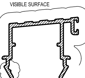
APT33 INTERNAL MID THRESHOLD Mass. 0,406 Kg/m Anod Per. 206 Paint Per. 100
