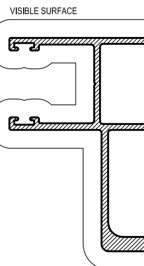
APT32 DG OXO MEDIUM STILE Mass. 1,622 Kg/m Anod Per. 367 Paint Per. 319 Ixx = 269.81 x 10 3 mm 4 Iyy = 223.66 x 10 3 mm 4
