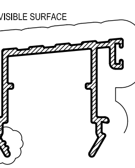
APT34 INTERNAL HIGH THRESHOLD Mass. 0,430 Kg/m Anod Per. 219 Paint Per. 100
