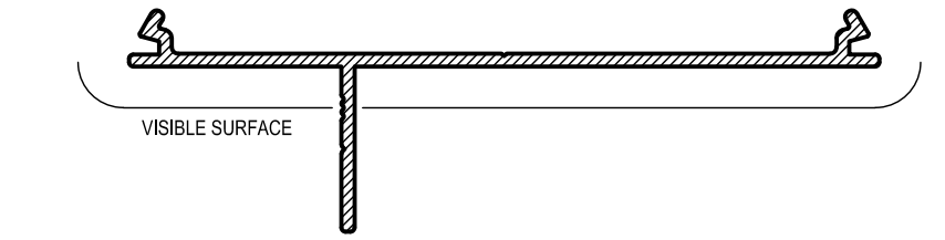
AS221 20mm REVEAL ADAPTOR Mass. 0,522 Kg/m Anod Per. 250 Paint Per. 100
