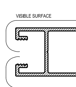
APT9 SG LOCK STILE Mass. 0,759 Kg/m Anod Per. 235 Paint Per. 151
