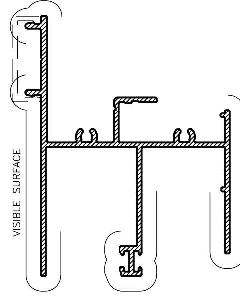
RSW50 FACE FIX HEAD Anod Per. 493 Paint Per. 184
