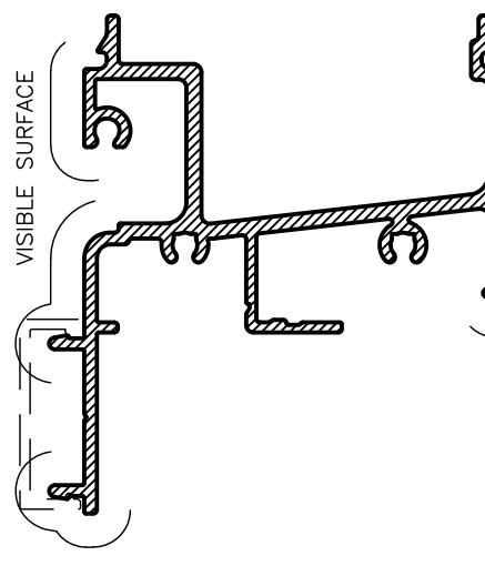
RSW54 FACE FIX SUMP SILL Anod Per. 434 Paint Per. 100
