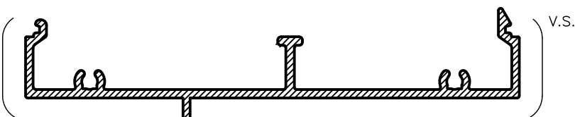
RSW927 SLIDING WINDOW RENDER FRAME Anod Per. 340 Paint Per. 100
