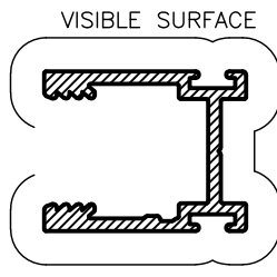
RSW104 STILE Anod Per. 159 Paint Per. 100
