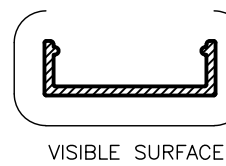
RSW53 FACE FIX COVER Anod Per. 100 Paint Per. 100
