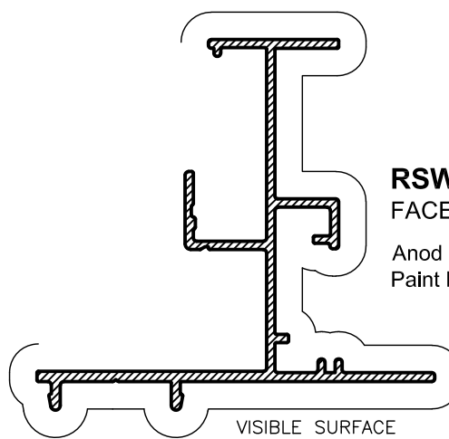
RSW53 FACE FIX COVER Anod Per. 100 Paint Per. 100
