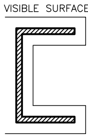
HD14 25.4 x 15.88 x 1.58mm CHANNEL Anod Per. 111 Paint Per. 100
