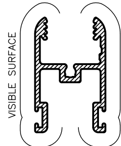
RSW105 RAIL Anod Per. 206 Paint Per. 146
