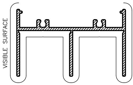
RSW160 SECONDARY GLAZED HEAD/JAMB Anod Per. 286 Paint Per. 202
