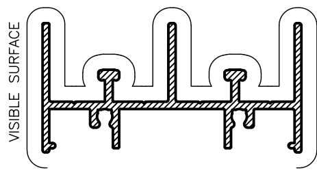
RSW161 SECONDARY GLAZED SILL Anod Per. 307 Paint Per. 136
