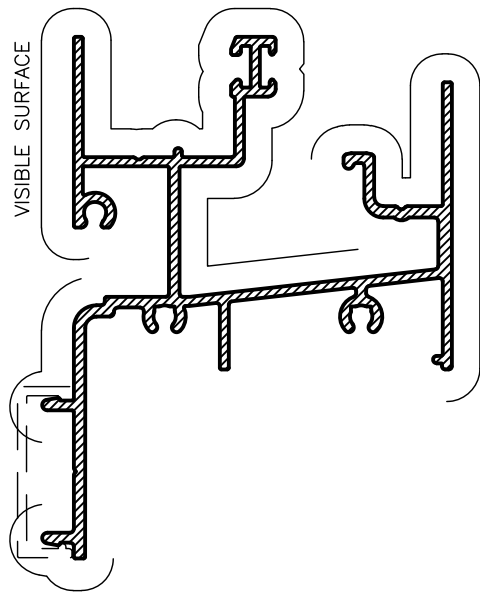
RSW55 ALT FACE FIX SILL Anod Per. 547 Paint Per. 309
