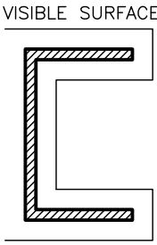
HD14 25.4 x 15.88 x 1.58mm CHANNEL Anod Per. 111 Paint Per. 100
