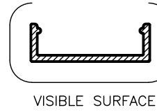
RSW53 FACE FIX COVER Anod Per. 100 Paint Per. 100
