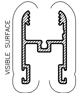
RSW105 RAIL Anod Per. 206 Paint Per. 146
