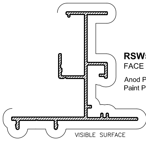
RSW53 FACE FIX COVER Anod Per. 100 Paint Per. 100
