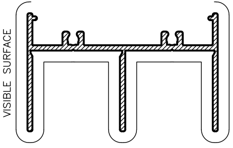
RSW160 SECONDARY GLAZED HEAD/JAMB Anod Per. 296 Paint Per. 202
