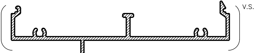
RSW927 SLIDING WINDOW RENDER FRAME Anod Per. 340 Paint Per. 100
