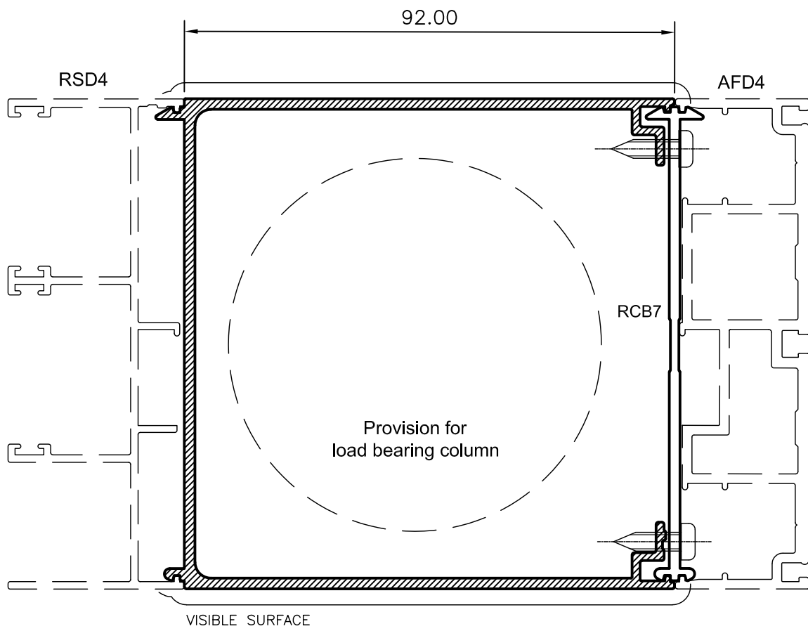
RCB19 92mm 180° COUPLING BAR Anod Per. 624 Paint Per.416
