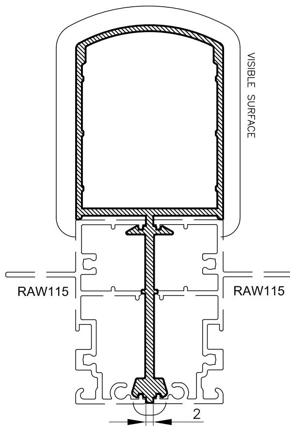
RCB9 HD 50mm COUPLING BAR Anod. 317 Paint Per. 137
