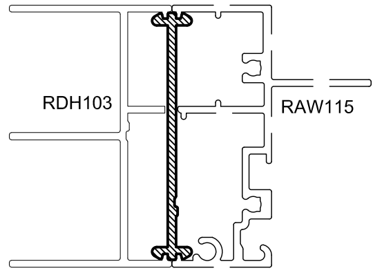
RCB1 50mm COUPLING BAR
