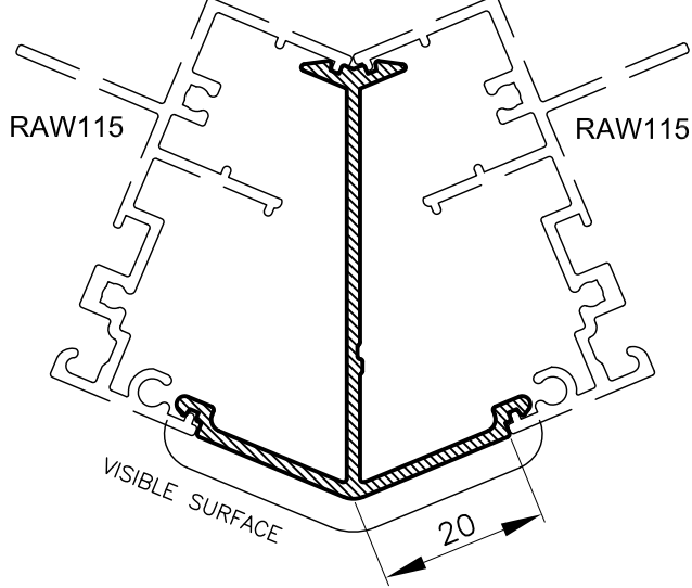
RCB2 50mm 135 Deg COUPLING BAR Anod Per. 232 Paint Per. 100
