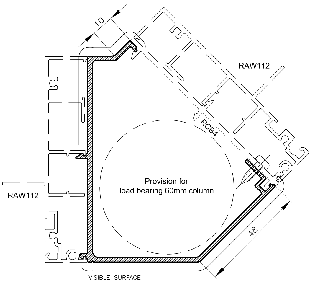
RCB5 92mm 135° DEG COUPLING BAR Anod Per. 483 Paint Per. 192
