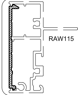
RCB15 50mm PLANT ON COUPLER Anod Per. 107 Paint Per. 100
