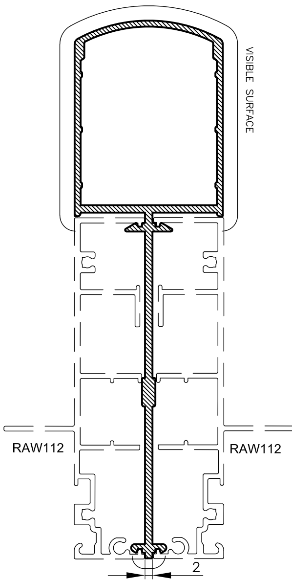
RCB13 HD 92mm COUPLER Anod Per. 404 Paint Per. 141
