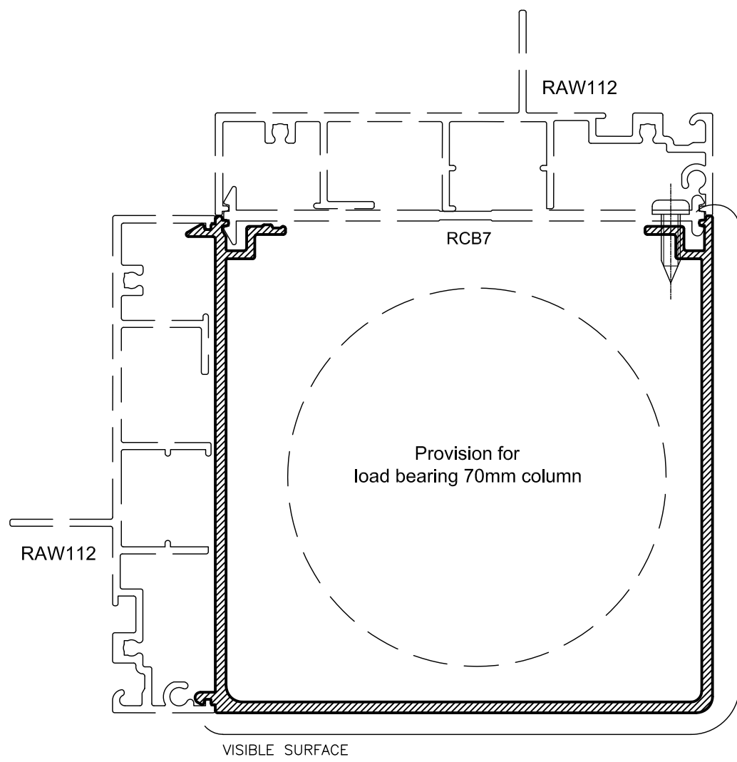
RCB18 92mm 90° DEG COUPLING BAR Anod Per. 624 Paint Per. 183
