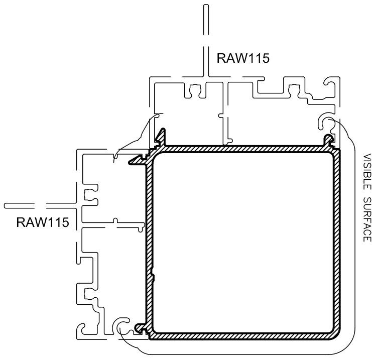
RCB3 50mm 90° COUPLING BAR Anod Per. 232 Paint Per. 122
