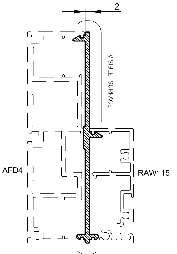
RCB8 50mm to 92mm COUPLER Anod Per. 226 Paint Per. 100
