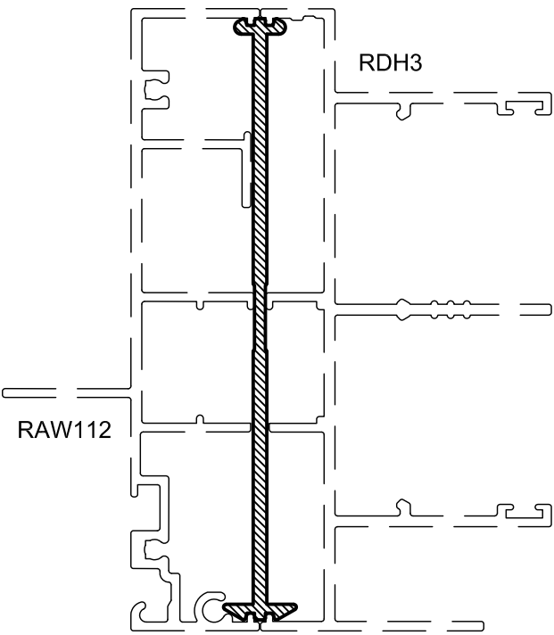
RCB7 92mm COUPLER Anod. Per. 226 Paint Per. 100
