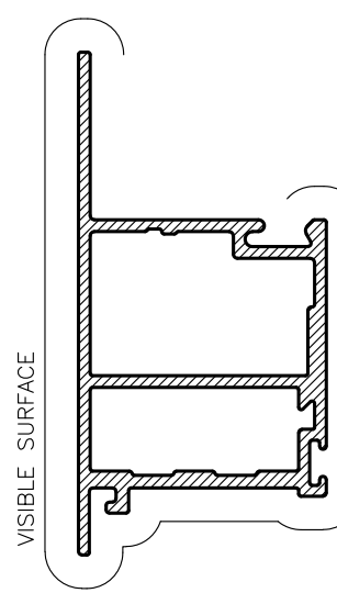
RAW51 60mm BEADED SASH Mass. 0.765 Kg/m Anod. Per. 204 Paint Per. 137
