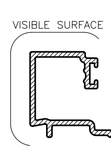
RAW18 THICK GLASS BEAD Anod Per. 144 Paint Per. 100
