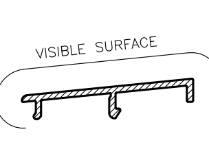
RAW20 INFILL Anod Per. 100 Paint Per. 100
