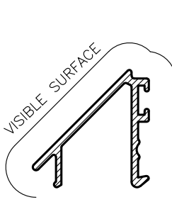
RAW7 SG BEAD Anod Per. 122 Paint Per. 100
