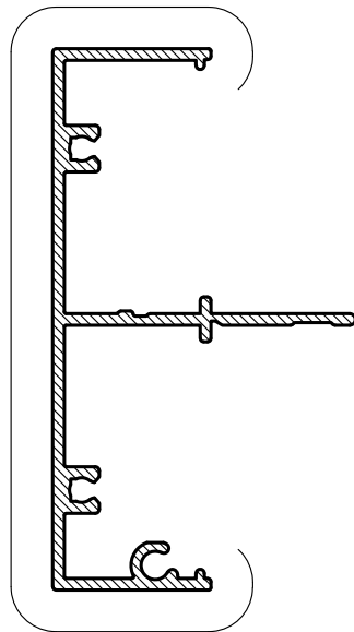
RAW656 65mm PLAIN FRAME Anod Per. 327 Paint Per. 105
