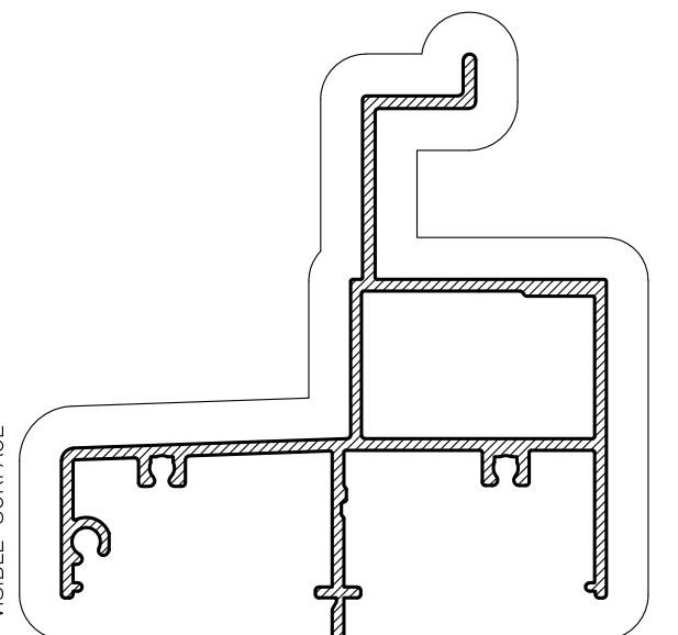
RAW651 65mm WINDER SILL Anod Per. 442 Paint Per. 214
