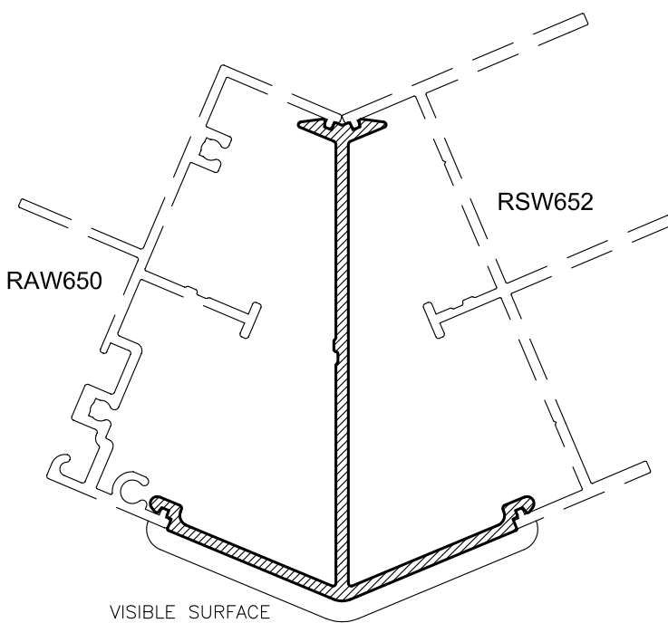
RCB21 65mm 135 DEG COUPLING BAR Anod Per. 291 Paint Per. 100
