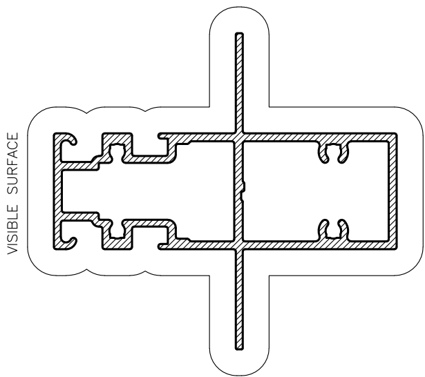
RAW653 MULLION / TRANSOM Anod Per. 302 Paint Per. 251
