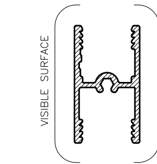
RAW22 30mm MID-RAIL Anod Per. 179 Paint Per. 100
