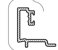
RAW10 DG BEAD Anod Per. 127 Paint Per. 100
