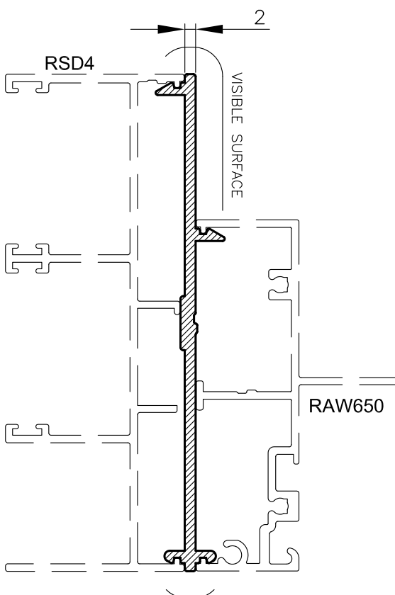
RCB22 65mm to 92mm COUPLER Anod Per. 227 Paint Per. 100
