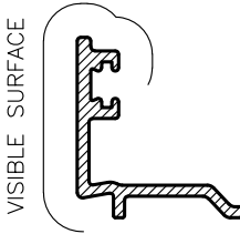
RAW36 24mm DG BEAD Anod Per. 102 Paint Per. 100
