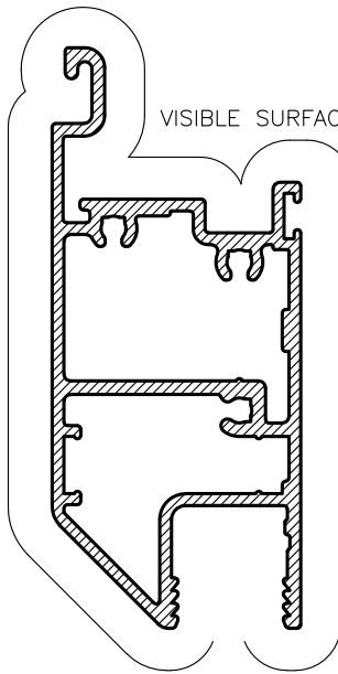
RAW29 SG 60mm HINGE SASH Anod Per. 267 Paint Per. 218
