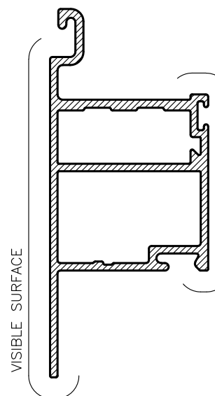
RAW50 60mm BEADED HINGE SASH Mass. 0.807 Kg/m Anod. Per. 230 Paint Per. 108
