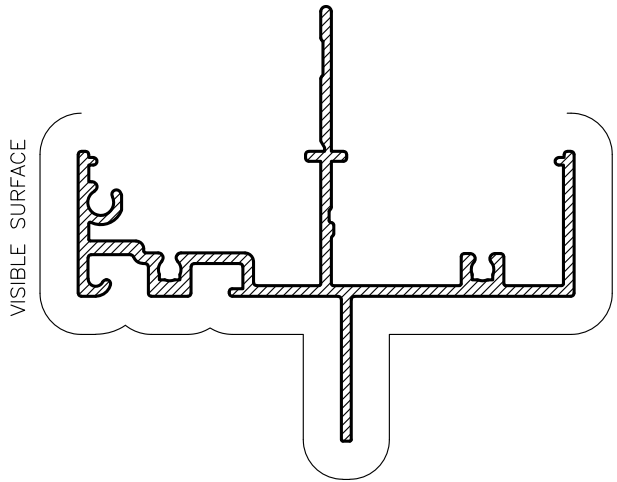
RAW650 FRAME Anod Per. 387 Paint Per. 142
