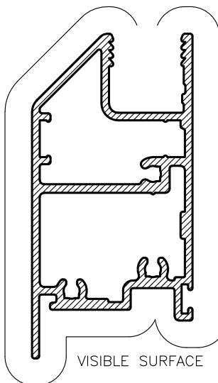
RAW30 SG 60mm SASH Anod Per. 233 Paint Per. 184
