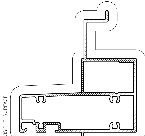
RAW652 65mm WINDER TRANSOM Anod Per. 350 Paint Per. 322
