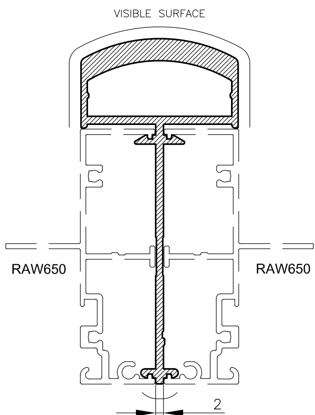
RCB23 HD 65mm COUPLER Anod Per. 288 Paint Per. 100
