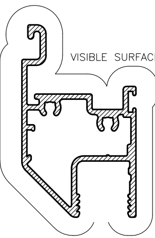
RAW27 SG HINGE SASH Anod Per. 229 Paint Per. 180
