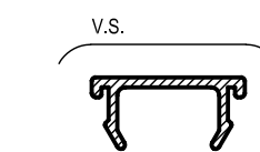
AS8C MULTI PURPOSE POCKET FILLER Mass. 0.113 Kg/m Anod. Per. 100 Paint Per. 100
