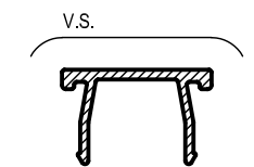
AS58 76mm FLUSH IN-FILL Mass. 0.138 Kg/m Anod. Per. 100 Paint Per. 100
