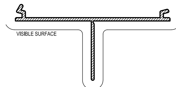
AS551 76mm FLASHING ADAPTOR Mass. 0.432 Kg/m Anod. Per. 222 Paint Per. 126
