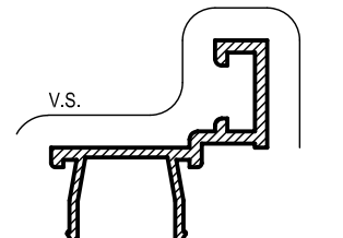
AS57 45mm DOOR STOP Mass. 0.248 Kg/m Anod. Per. 141 Paint Per. 100
