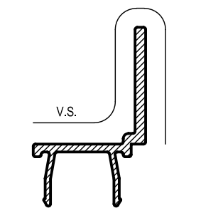
AS585 AWNING SASH ADAPTOR Mass. 0.268 Kg/m Anod. Per. 131 Paint Per. 100
