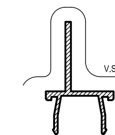
AS581 35mm SASH ADAPTOR Mass. 0.206 Kg/m Anod. Per. 121 Paint Per. 100
