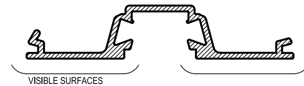
AS554 GLAZING ADAPTOR Mass. 0.533 Kg/m Anod. Per. 233 Paint Per. 100 I_{xx} = 73.30 \times 10^{-3} \text{ mm}^4
