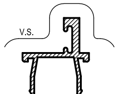
AS56 35mm DOOR STOP Mass. 0.205 Kg/m Anod. Per. 111 Paint Per. 100
