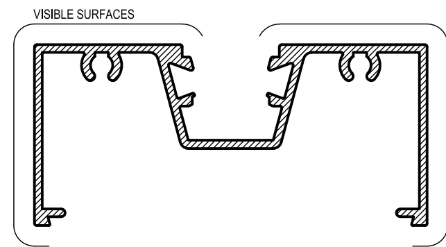
AS53 76mm SILL BEAD Mass. 0.295 Kg/m Anod. Per. 155 Paint Per. 100
