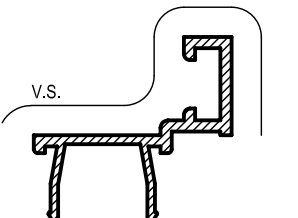
AS57 45mm DOOR STOP Mass. 0.248 Kg/m Anod. Per. 141 Paint Per. 100
