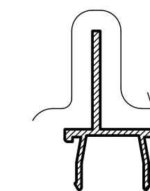
AS581 35mm SASH ADAPTOR Mass. 0.206 Kg/m Anod. Per. 121 Paint Per. 100
