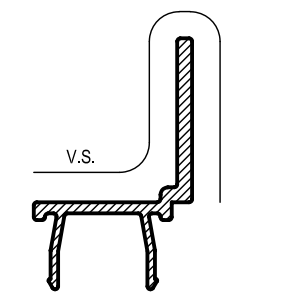
AS585 AWNING SASH ADAPTOR Mass. 0.268 Kg/m Anod. Per. 131 Paint Per. 100
