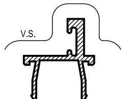
AS56 35mm DOOR STOP Mass. 0.205 Kg/m Anod. Per. 111 Paint Per. 100
