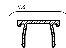
AS58 76mm FLUSH IN-FILL Mass. 0.138 Kg/m Anod. Per. 100 Paint Per. 100
