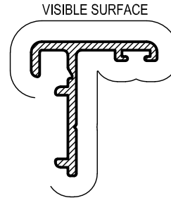
TM5 SECURITY MULLION Anod. Per. 126 Paint Per. 100
