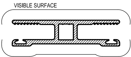
ADF8 ECO-GARD MID-RAIL Anod. Per. 235 Paint Per. 114
