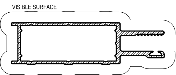
ADF5 ECO-GARD DOOR FRAME Anod. Per. 238 Paint Per. 177
