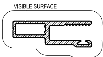
AWF5RB ECO-GARD 9mm FRAME Anod. Per. 152 Paint Per. 100
