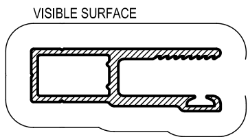
AWF5 ECO-GARD WINDOW FRAME Anod. Per. 153 Paint Per. 100
