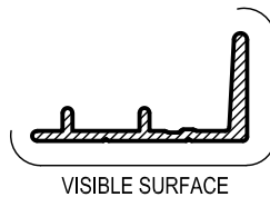
HD9 FRAME INTERLOCK Anod. Per. 100 Paint Per. 100
