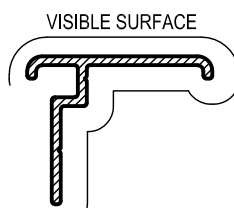
TM18 OFFSET T MULLION Anod. Per. 100 Paint Per. 100
