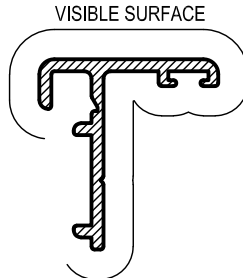
TM5 SECURITY MULLION Anod. Per. 126 Paint Per. 100
