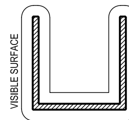
HD6 CHANNEL 25 x 25 x 1.6mm Anod. Per. 146 Paint Per. 146
