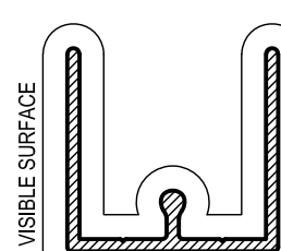
ST8 BOTTOM SLIDING TRACK Anod. Per. 160 Paint Per. 138
