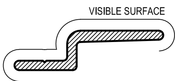
HD28 HEAVY DUTY DEEP INTERLOCK Anod. Per. 100 Paint Per. 100
