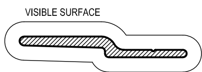
HD22 HEAVY DUTY STEPPED INTERLOCK Anod. Per. 100 Paint Per. 100
