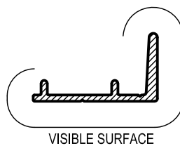
HD29 ALTITUDE / CARINYA INTERLOCK Anod. Per. 100 Paint Per. 100
