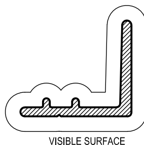
HD23 HEAVY DUTY FRAME INTERLOCK Anod. Per. 114 Paint Per. 114
