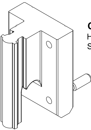
CP103 HOOK BRACKET SET
