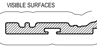
UCW165 136mm SSG 32-34mm IGU GLAZING BEAD Mass. 0.463 Kg/m Anod. Per. 115 Paint Per. 100
