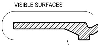
UCW158 136mm SSG 28-30mm IGU GLAZING SEAT Mass. 0.398 Kg/m Anod. Per. 89 Paint Per. 100
