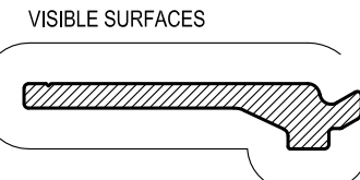
UCW159 136mm SSG 32-34mm IGU GLAZING SEAT Mass. 0.422 Kg/m Anod. Per. 95 Paint Per. 100
