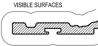
UCW164 136mm SSG 28-30mm IGU GLAZING BEAD Mass. 0.428 Kg/m Anod. Per. 106 Paint Per. 100
