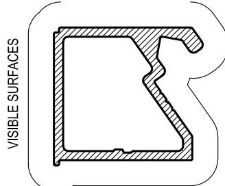
UCW163 136mm SSG SINGLE GLAZE ADAPTOR 26mm Mass. 0.560 Kg/m Anod. Per. 124 Paint Per. 100
