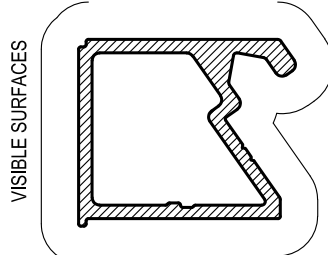
UCW162 136mm SSG SINGLE GLAZE ADAPTOR 24mm Mass. 0.540 Kg/m Anod. Per. 120 Paint Per. 100
