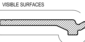
UCW160 136mm SSG 36-38mm IGU GLAZING SEAT Mass. 0.446 Kg/m Anod. Per. 101 Paint Per. 100
