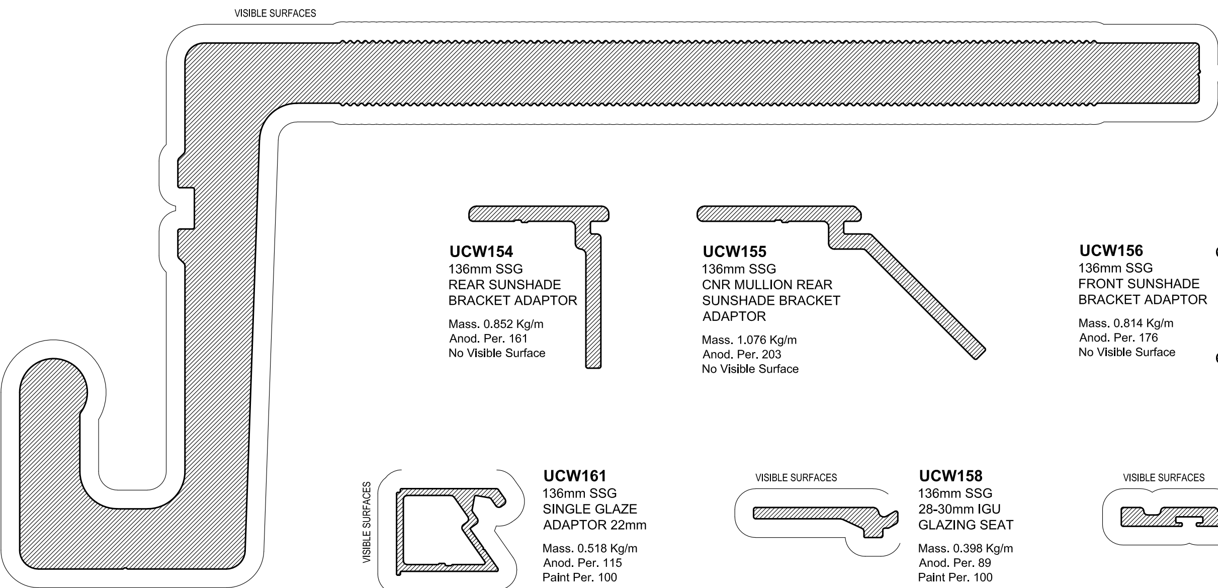
UCW181 136mm SSG STRUCTURAL DROP DOWN FLOOR BRACKET Mass. 21.795 Kg/m Anod. Per. 1067 Paint Per. 1067
