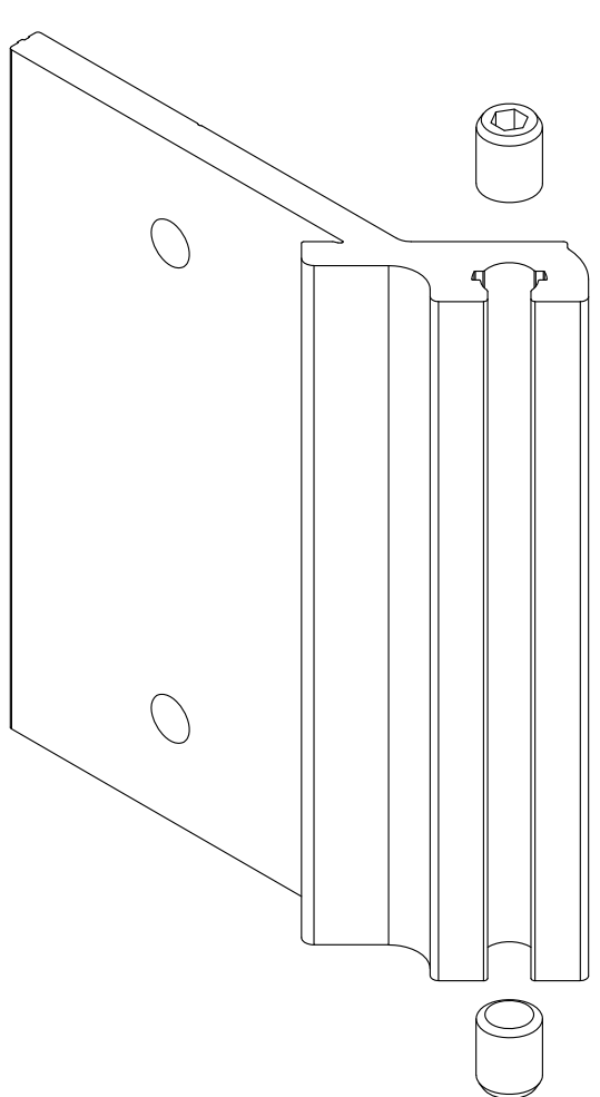
CP102 CORNER MULLION BRACKET SET
