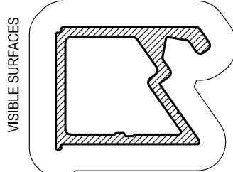
UCW161 136mm SSG SINGLE GLAZE ADAPTOR 22mm Mass. 0.518 Kg/m Anod. Per. 115 Paint Per. 100
