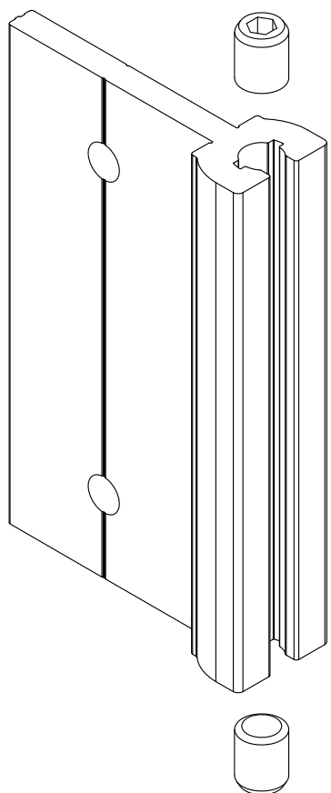
CP101 MULLION BRACKET SET
