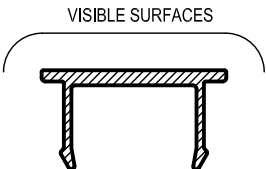
ME8 POCKET FILLER Mass. 0.181 Kg/m Anod. Per. 100 Paint Per. 100
