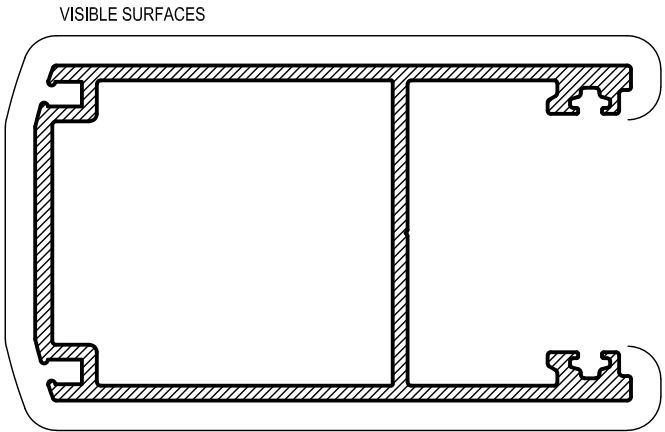
SE422 DG LOCK STILE / PIVOT STILE Mass. 1.542 Kg/m Anod. Per. 366 Paint Per. 233 I_{xx} = 195.1 \times 10^3 \text{ mm}^4
