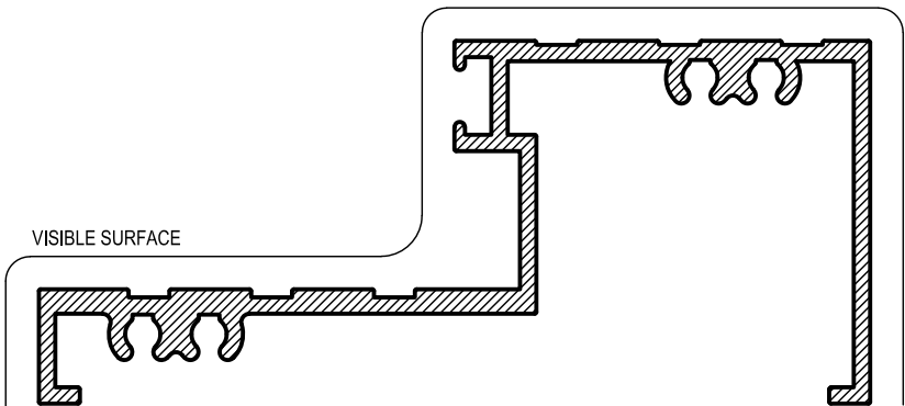
AS2366 45mm DOOR THRESHOLD OUTWARD OPENING Mass. 1.552 Kg/m Anod. Per. 491 Paint Per. 239
