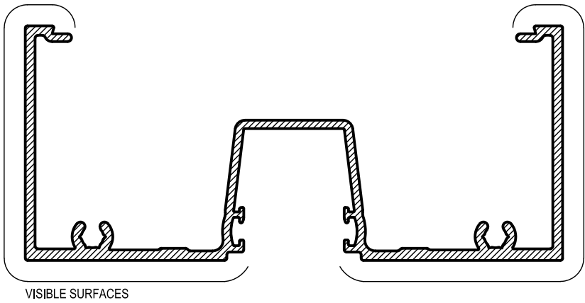
ME1 FRAME / JAMB Mass. 1.365 Kg/m Anod. Per. 560 Paint Per. 182 I_{xx} = 695.7 \times 10^3 \text{ mm}^4
