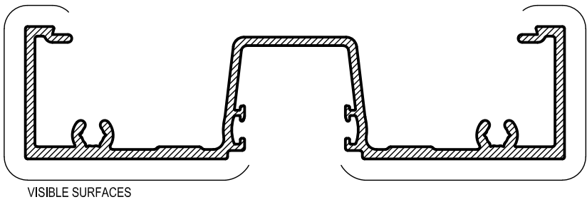
ME24 25mm NARROW FRAME Mass. 1.140 Kg/m Anod. Per. 468 Paint Per. 127
