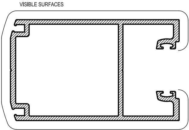
SE22 LOCK STILE / PIVOT STILE Mass. 1.564 Kg/m Anod. Per. 392 Paint Per. 236 I_{xx} = 183.4 \times 10^3 \text{ mm}^4
