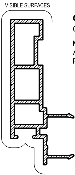
GSS1 GAS STRUT CLIP-ON STOP Mass. 0.799 Kg/m Anod. Per. 228 Paint Per. 100
