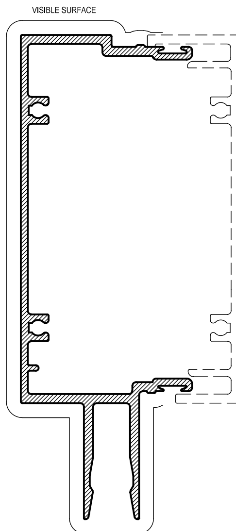
AS203 101.6mm DG SPLIT MULLION (MALE) Mass. 1.701 Kg/m Anod. Per. 589 Paint Per. 235 I_{xx} = 1242.73 \times 10^3 \text{ mm}^4 I_{yy} = 125.61 \times 10^3 \text{ mm}^4
