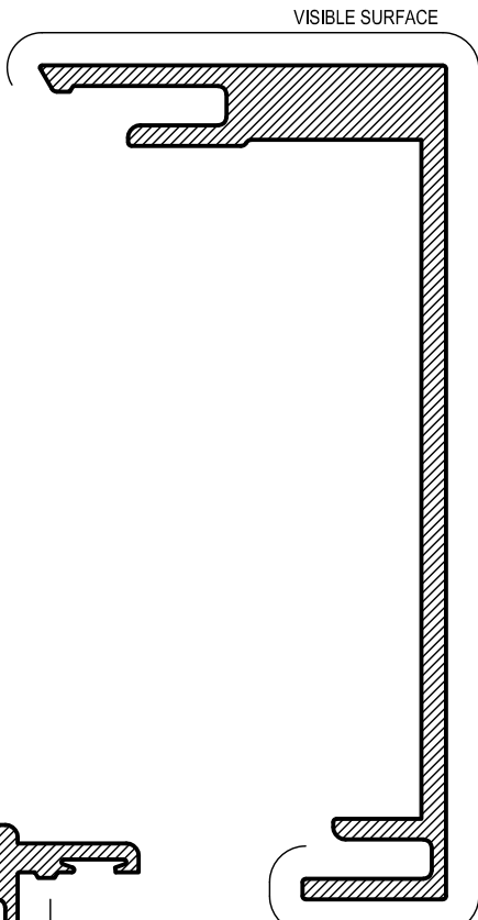
AS112 HEAVY SPLIT MULLION Mass. 1.804 Kg/m Anod. Per. 377 Paint Per. 174 I_{xx} = 847.74 \times 10^3 \text{ mm}^4 I_{yy} = 100.62 \times 10^3 \text{ mm}^4
