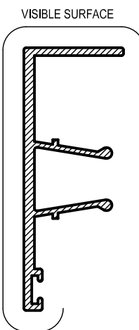
AS105 SNAP ADAPTOR Mass. 0.443 Kg/m Anod. Per. 211 Paint Per. 100
