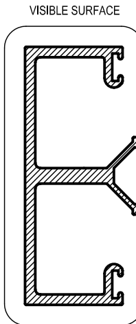
AS113 DEEP ADAPTOR Mass. 0.749 Kg/m Anod. Per. 235 Paint Per. 100
