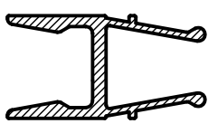
AS126 DOUBLE SNAP GLAZING ADAPTOR Mass. 0.299 Kg/m Anod. Per. 147 No Visible Surface
