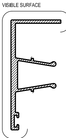
AS125 SNAP ADAPTOR WITH LEG Mass. 0.515 Kg/m Anod. Per. 232 Paint Per. 100
