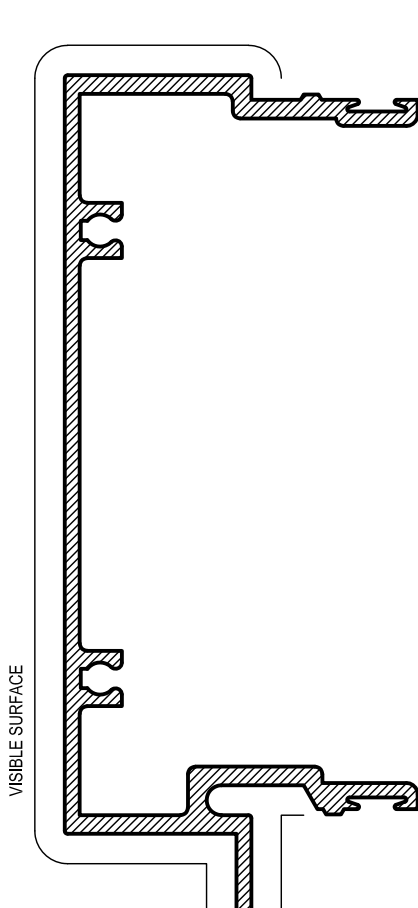
AS115 STRUCTURAL SPLIT MULLION (MALE) Mass. 1.491 Kg/m Anod. Per. 502 Paint Per. 163 I_{xx} = 890.33 \times 10^3 \text{ mm}^4 I_{yy} = 111.53 \times 10^3 \text{ mm}^4
