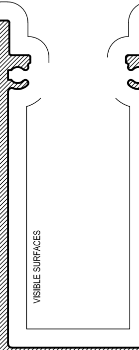
ASGR8 SLOTTED GRATE THRESHOLD Mass. 0.364 Kg/m Anod. Per. 105 Paint Per. 100 PREPUNCHED AND CLEAR ANODISED
