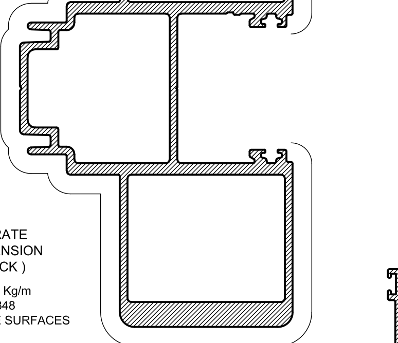
HS216 DG HD MALE MEETING STILE Mass. 3.946 Kg/m Anod. Per. 498 Paint Per. 346 Ixx = 2623.68 x 10 3 mm 4
