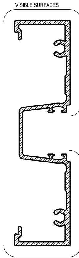
ME24 25mm NARROW FRAME Mass. 1.140 Kg/m Anod. Per. 468 Paint Per. 127
