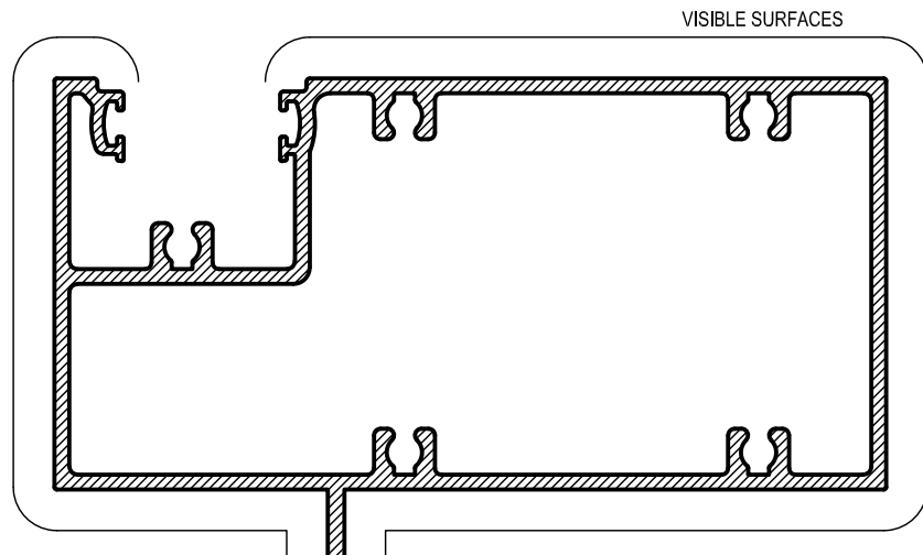
HE324 TRANSOM SG 35mm SASH Mass. 2.053 Kg/m Anod. Per. 455 Paint Per. 316 Ixx = 884.68 x 10 3 mm 4
