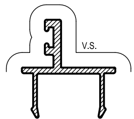
ME40 40mm DOOR STOP Mass. 0.271 Kg/m Anod. Per. 136 Paint Per. 100
