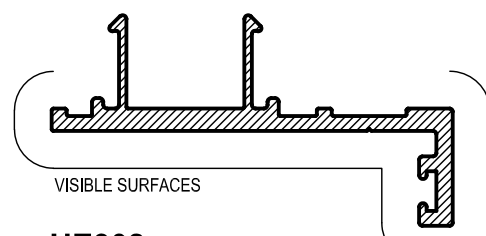
HE308 45mm DOOR STOP Mass. 0.579 Kg/m Anod. Per. 212 Paint Per. 100
