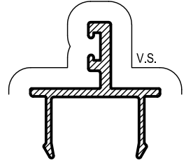
ME45 45mm DOOR STOP Mass. 0.271 Kg/m Anod. Per. 136 Paint Per. 100
