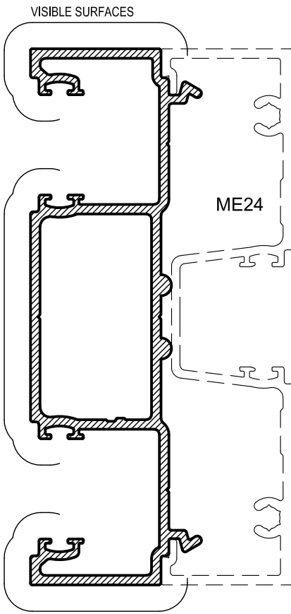
HE910 ACOUSTIC DOOR JAMB ADAPTOR Mass. 1.427 Kg/m Anod. Per. 480 Paint Per. 125 Ixx = 572.12 x 10 3 mm 4
