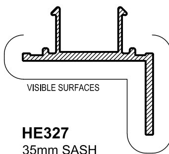
HE327 35mm SASH ADAPTOR Mass. 0.395 Kg/m Anod. Per. 171 Paint Per. 100
