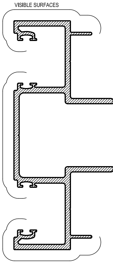
HE902 ACOUSTIC MALE MULLION Mass. 1.734 Kg/m Anod. Per. 607 Paint Per. 143 Ixx = 682.94 x 10 3 mm 4
