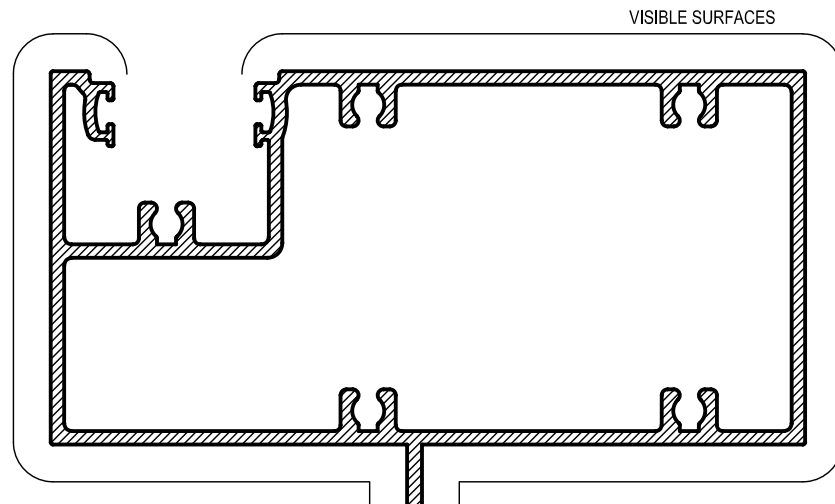
HE325 TRANSOM SG 50mm SASH Mass. 2.064 Kg/m Anod. Per. 459 Paint Per. 320 Ixx = 877.36 x 10 3 mm 4
