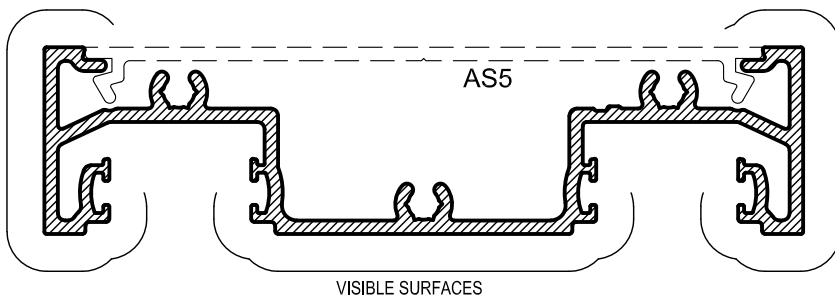
HE911 25mm ACOUSTIC FRAME Mass. 1.260 Kg/m Anod. Per. 535 Paint Per. 154
