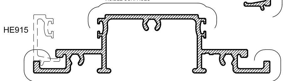
HE915 25mm ACOUSTIC SILL BEAD Mass. 0.204 Kg/m Anod. Per. 100 Paint Per. 100
