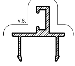
ME7 45mm DOOR STOP Mass. 0.275 Kg/m Anod. Per. 138 Paint Per. 100
