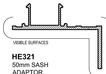
HE321 50mm SASH ADAPTOR Mass. 0.470 Kg/m Anod. Per. 205 Paint Per. 100
