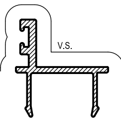
ME35 35mm DOOR STOP Mass. 0.271 Kg/m Anod. Per. 136 Paint Per. 100
