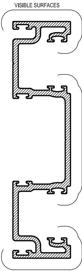
HE903 ACOUSTIC FEMALE MULLION Mass. 1.482 Kg/m Anod. Per. 544 Paint Per. 125 Ixx = 665.42 x 10 3 mm 4
