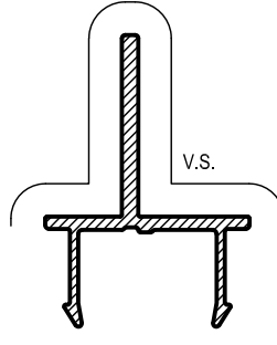
ME30 50mm SASH ADAPTOR Mass. 0.293 Kg/m Anod. Per. 143 Paint Per. 100
