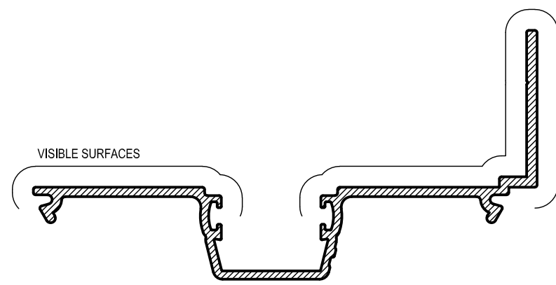
ME15 FLASHING ADAPTOR Mass. 0.750 Kg/m Anod. Per. 354 Paint Per. 145
