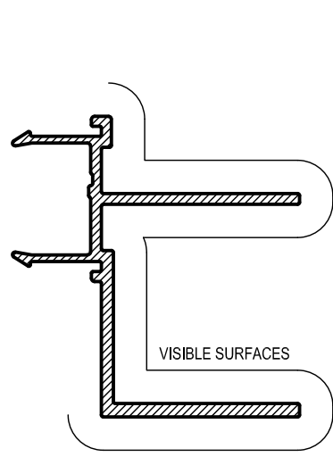
VM76 SASH RECEIVER ADAPTOR Mass. 0.734 Kg/m Anod. Per. 346 Paint Per. 225
