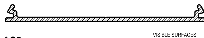
AS5 FLUSH ADAPTOR Mass. 0.500 Kg/m Anod. Per. 213 Paint Per. 100 Ixx = 150.5 x 10 3 mm 4
