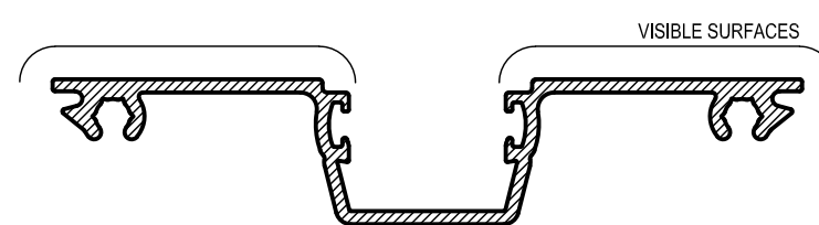
ME4 GLAZING ADAPTOR Mass. 0.685 Kg/m Anod. Per. 303 Paint Per. 100 Ixx = 187.7 x 10 3 mm 4
