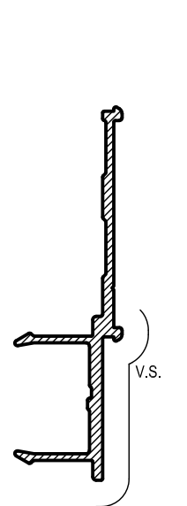
AF54 McARTHUR EVO SLIM LOUVRE ADAPTOR Mass. 0.337 Kg/m Anod. Per. 171 Paint Per. 100
