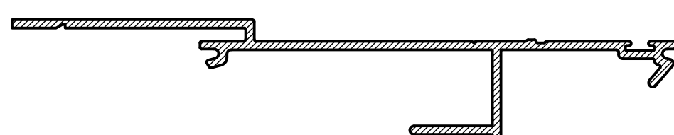
ME19 100mm FIXING LEG ADAPTOR Mass. 0.973 Kg/m Anod. Per. 391 Paint Per. 100
