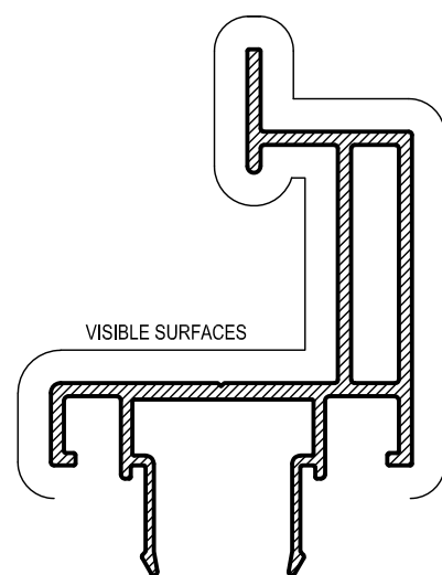
ASW118 McARTHUR EVO PROTILT AWNING ADAPTOR Mass. 0.858 Kg/m Anod. Per. 337 Paint Per. 172
