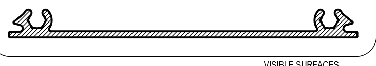
AS5F FLUSH ADAPTOR WITH SCREW FLUTES Mass. 0.538 Kg/m Anod. Per. 231 Paint Per. 100 Ixx = 180.0 x 10 3 mm 4
