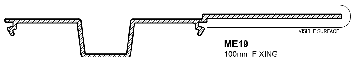
AS222 101.6mm 13mm PLASTERBOARD ADAPTOR Mass. 1.043 Kg/m Anod. Per. 395 No Visible Surface
