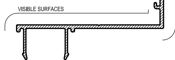
AF45 McARTHUR EVO LOUVRE SILL ADAPTOR Mass. 0.556 Kg/m Anod. Per. 293 Paint Per. 135
