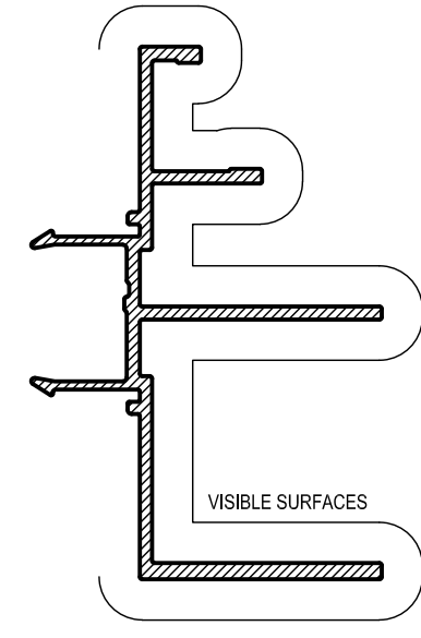
VM75 SASH SCREEN RECEIVER ADAPTOR Mass. 0.734 Kg/m Anod. Per. 346 Paint Per. 225
