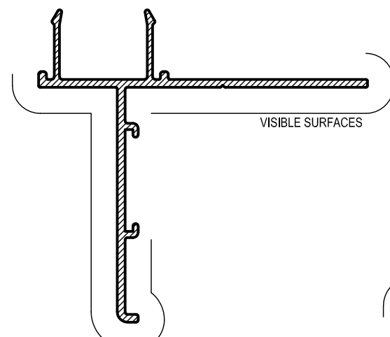
AF44 McARTHUR EVO LOUVRE HEAD ADAPTOR Mass. 0.556 Kg/m Anod. Per. 293 Paint Per. 138
