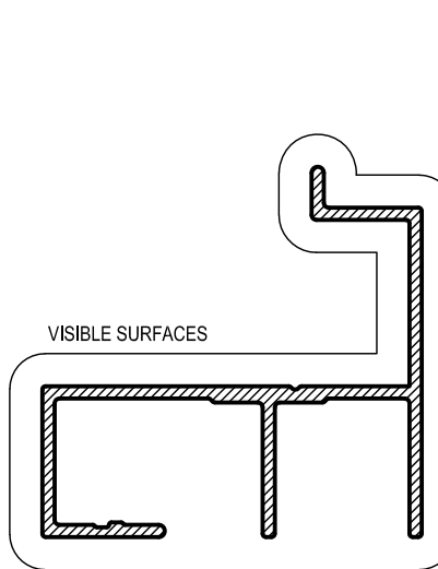
ASW43 AWNING WINDER ADAPTOR Mass. 0.624 Kg/m Anod. Per. 299 Paint Per. 160
