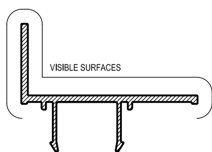
ME32 35mm SASH ADAPTOR Mass. 0.430 Kg/m Anod. Per. 204 Paint Per. 100
