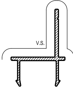
ME33 443 SASH ADAPTOR Mass. 0.268 Kg/m Anod. Per. 143 Paint Per. 100
