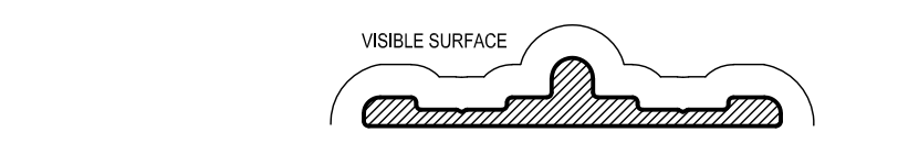
AD775 PLANT ON TRACK Mass. 0.442 Kg/m Anod. Per. 117 Paint Per. 100
