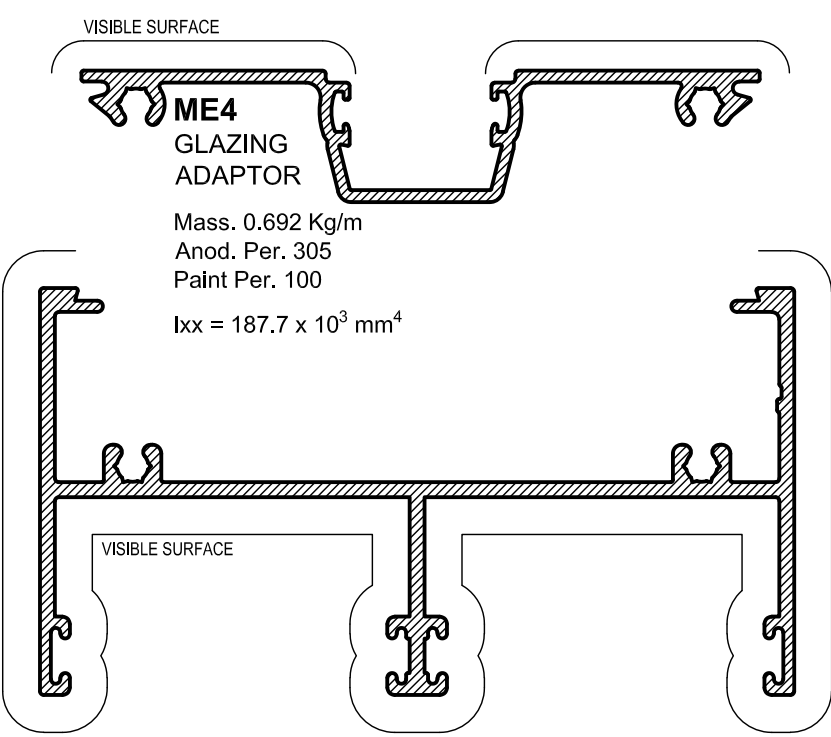
AD841 DOUBLE HEAD /JAMB Mass. 1.549 Kg/m Anod. Per. 584 Paint Per. 359 Ixx = 829.30 x 10 3 mm 4 Iyy = 104.80 x 10 3 mm 4
