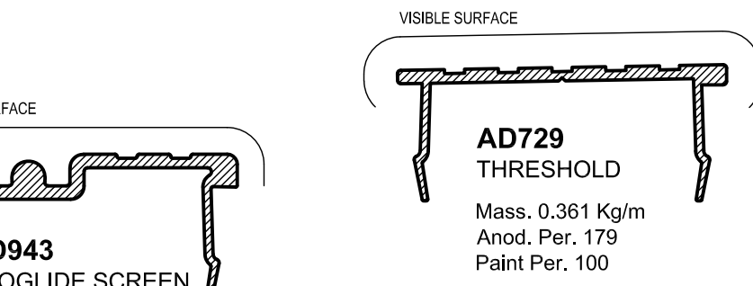
AD883S ALT. HP DOUBLE TRACK SILL Mass. 1.928 Kg/m Anod. Per. 696 Paint Per. 499
