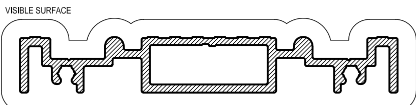
AD783 RECESSED DOUBLE TRACK Mass. 1.383 Kg/m Anod. Per. 366 Paint Per. 165
