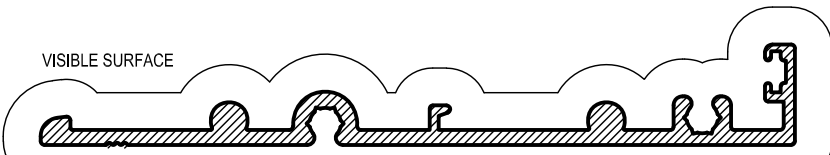
AD762 DISABLED SILL Mass. 0.822 Kg/m Anod. Per. 299 Paint Per. 189
