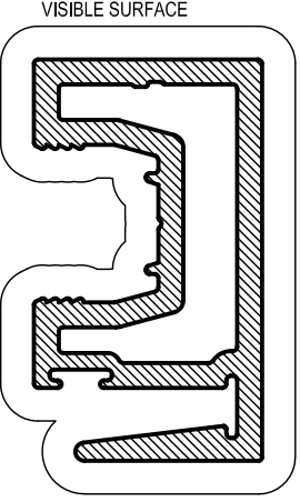
AD981 18mm POCKET SLIM INTERLOCK Mass. 1.456 Kg/m Anod. Per. 236 Paint Per. 236 Ixx = 39.38 x 10 3 mm 4
