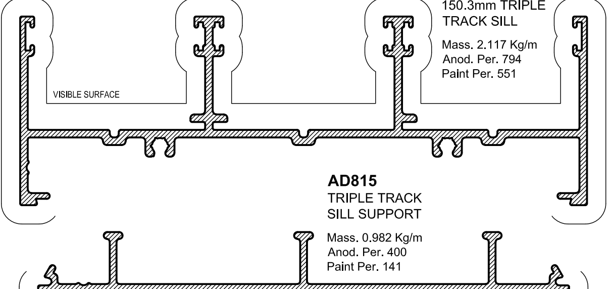
AD851R 150.3mm TRIPLE FRAME / JAMB Mass. 2.040 Kg/m Anod. Per. 776 Paint Per. 514 Ixx = 2068.02 x 10 3 mm 4 Iyy = 126.86 x 10 3 mm 4
