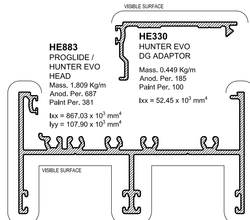
HE332 HUNTER EVO SG ADAPTOR Mass. 0.536 Kg/m Anod. Per. 221 Paint Per. 100 Ixx = 111.89 x 10 3 mm 4
