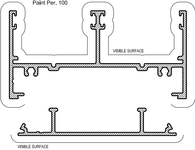
AD812 TRACK Mass. 0.271 Kg/m Anod. Per. 118 Paint Per. 100
