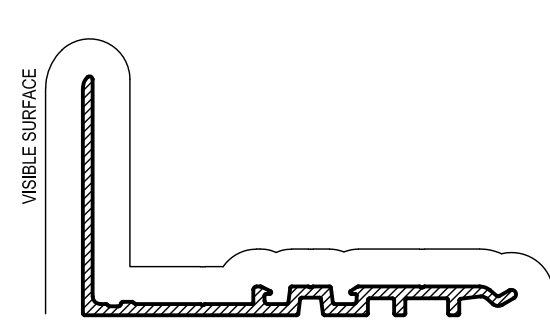
SDH019 JAMB OUTER LEG 18mm Mass. 0.401 Kg/m Anod. Per. 192 Paint Per. 121
