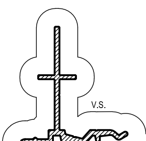
SDH016 JAMB ADD-ON LEG 10mm Mass. 0.272 Kg/m Anod. Per. 148 Paint Per. 107
