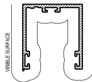
SDH014 HEAD 10mm Mass. 0.373 Kg/m Anod. Per. 200 Paint Per. 139
