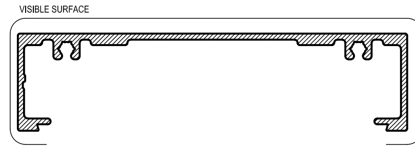
AS23 25mm PLAIN FRAME Mass. 0.961 Kg/m Anod. Per. 367 Paint Per. 163 Ixx = 513.44 x 10 3 mm 4
