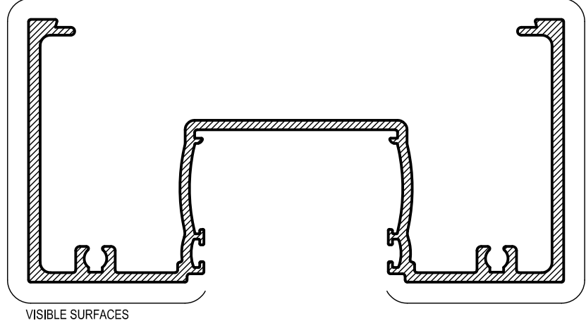
ECO201 101.6mm DG FRAME Mass. 1.592 Kg/m Anod. Per. 602 Paint Per. 180 Ixx = 858.76 x 10 3 mm 4 Iyy = 142.04 x 10 3 mm 4
