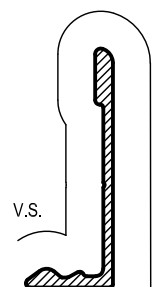
SDH002 JAMB INNER LEG Mass. 0.181 Kg/m Anod. Per. 100 Paint Per. 100
