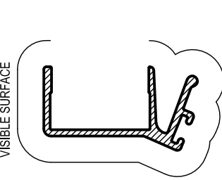
SDH022 INTERLOCK 18mm Mass. 0.229 Kg/m Anod. Per. 135 Paint Per. 100
