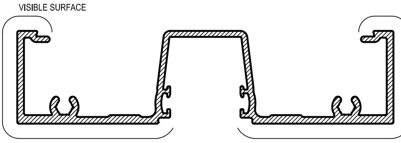
ME22 25mm NARROW FRAME Mass. 1.155 Kg/m Anod. Per. 475 Paint Per. 143
