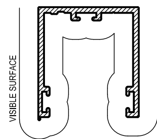
SDH014 HEAD 10mm Mass. 0.373 Kg/m Anod. Per. 200 Paint Per. 139
