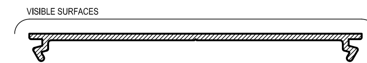
AS5 FLUSH ADAPTOR Mass. 0.500 Kg/m Anod. Per. 213 Paint Per. 100
