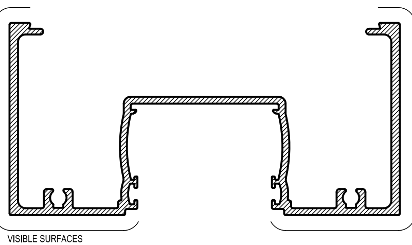
ECO201 101.6mm DG FRAME Mass. 1.592 Kg/m Anod. Per. 602 Paint Per. 180 Ixx = 858.76 x 10 3 mm 4 Iyy = 142.04 x 10 3 mm 4
