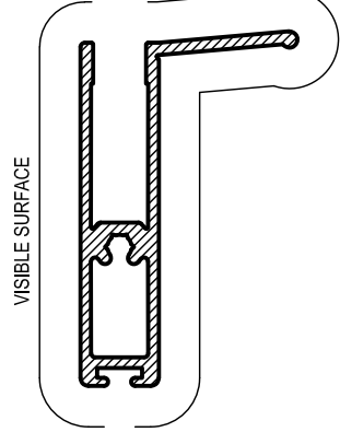
SDH008 LIFT RAIL 6mm Mass. 0.477 Kg/m Anod. Per. 192 Paint Per. 121
