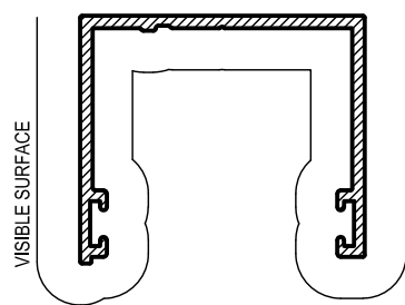
SDH018 HEAD 18mm Mass. 0.391 Kg/m Anod. Per. 205 Paint Per. 150
