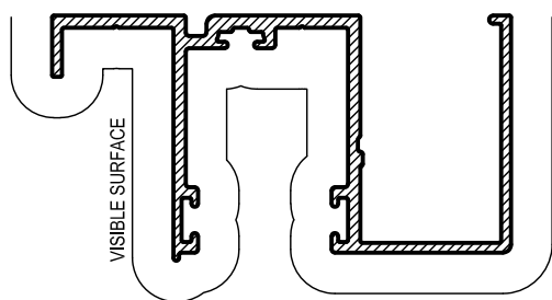
SDH010 HEAD 6mm (NO LEGS) Mass. 0.605 Kg/m Anod. Per. 329 Paint Per. 179
