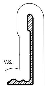
SDH002 JAMB INNER LEG Mass. 0.181 Kg/m Anod. Per. 100 Paint Per. 100
