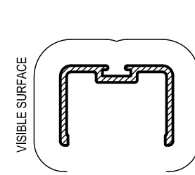
SDH021 RAIL 18mm Mass. 0.176 Kg/m Anod. Per. 110 Paint Per. 100
