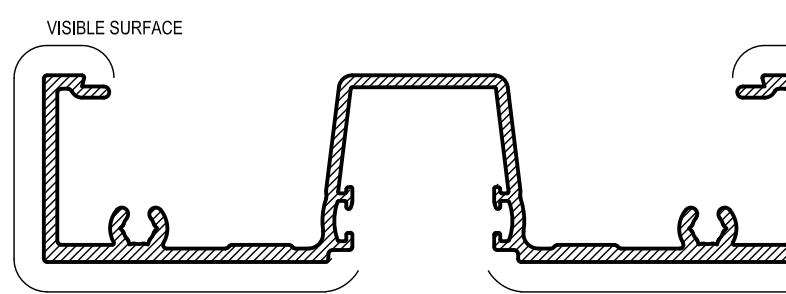
ME22 25mm NARROW FRAME Mass. 1.155 Kg/m Anod. Per. 475 Paint Per. 143
