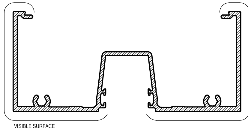
ME1 FRAME / JAMB Mass. 1.365 Kg/m Anod. Per. 560 Paint Per. 182 Ixx = 695.7 x 10 3 mm 4
