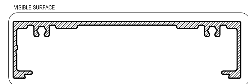
AS23 25mm PLAIN FRAME Mass. 0.961 Kg/m Anod. Per. 367 Paint Per. 163 Ixx = 513.44 x 10 3 mm 4
