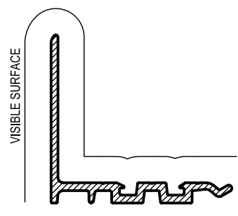
SDH005 JAMB OUTER LEG 6mm Mass. 0.289 Kg/m Anod. Per. 155 Paint Per. 100
