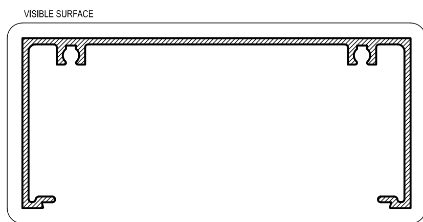
AS24 PLAIN FRAME Mass. 1.010 Kg/m Anod. Per. 201 Paint Per. 180 Ixx = 606.3 x 10 3 mm 4
