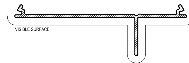
AS221 20mm REVEAL ADAPTOR Mass. 0.522 Kg/m Anod. Per. 250 Paint Per. 100
