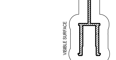
SDH003 JAMB RUNNER Mass. 0.226 Kg/m Anod. Per. 118 Paint Per. 100
