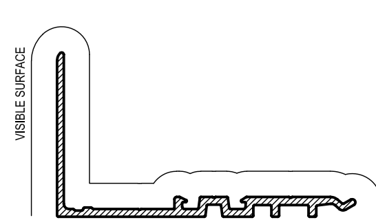
SDH019 JAMB OUTER LEG 18mm Mass. 0.401 Kg/m Anod. Per. 207 Paint Per. 121
