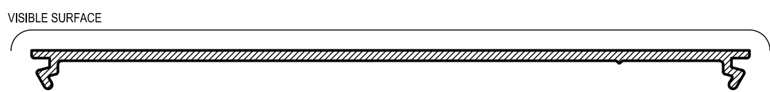
AS605 150mm FLUSH ADAPTOR Mass. 0.810 Kg/m Anod. Per. 310 Paint Per. 140 Ixx = 539.1 x 10 3 mm 4
