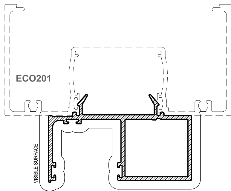
ECO201 SDH HEAD 18mm ADAPTOR Mass. 0.941 Kg/m Anod. Per. 316 Paint Per. 179
