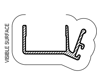
SDH022 INTERLOCK 18mm Mass. 0.229 Kg/m Anod. Per. 135 Paint Per. 100
