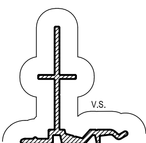
SDH016 JAMB ADD-ON LEG 10mm Mass. 0.272 Kg/m Anod. Per. 148 Paint Per. 107
