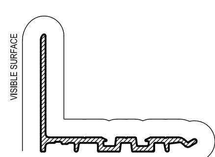
SDH015 JAMB OUTER LEG 10mm Mass. 0.329 Kg/m Anod. Per. 175 Paint Per. 103
