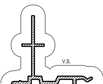
SDH020 ADD-ON LEG 18mm Mass. 0.305 Kg/m Anod. Per. 167 Paint Per. 103
