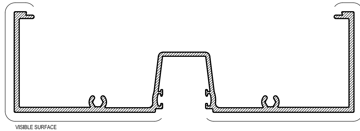
ME61 FRAME / JAMB Mass. 1.795 Kg/m Anod. Per. 650 Paint Per. 230 Ixx = 1837.1 x 10 3 mm 4
