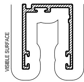
SDH011 6mm ACOUSTIC HEAD/SILL Mass. 0.349 Kg/m Anod. Per. 189 Paint Per. 132
