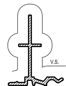
SDH006 JAMB ADD-ON LEG 6mm Mass. 0.245 Kg/m Anod. Per. 138 Paint Per. 106
