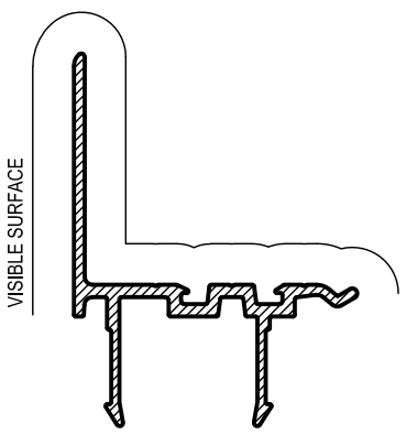
SDH012 JAMB OUTER 6mm CLIP IN Mass. 0.373 Kg/m Anod. Per. 209 Paint Per. 100
