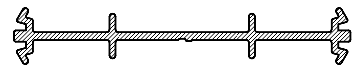
AS60 100mm INTERNAL COUPLER Mass. 0.752 Kg/m Anod. Per. 281 No Visible Surface Ixx = 249 x 10 3 mm 4
