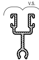
SDH026 BAL40 STILE 6mm Mass. 0.208 Kg/m Anod. Per. 125 Paint Per. 100
