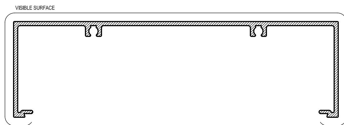
AS74 150mm PLAIN FRAME Mass. 1.397 Kg/m Anod. Per. 541 Paint Per. 249 Ixx = 1620.6 x 10 3 mm 4
