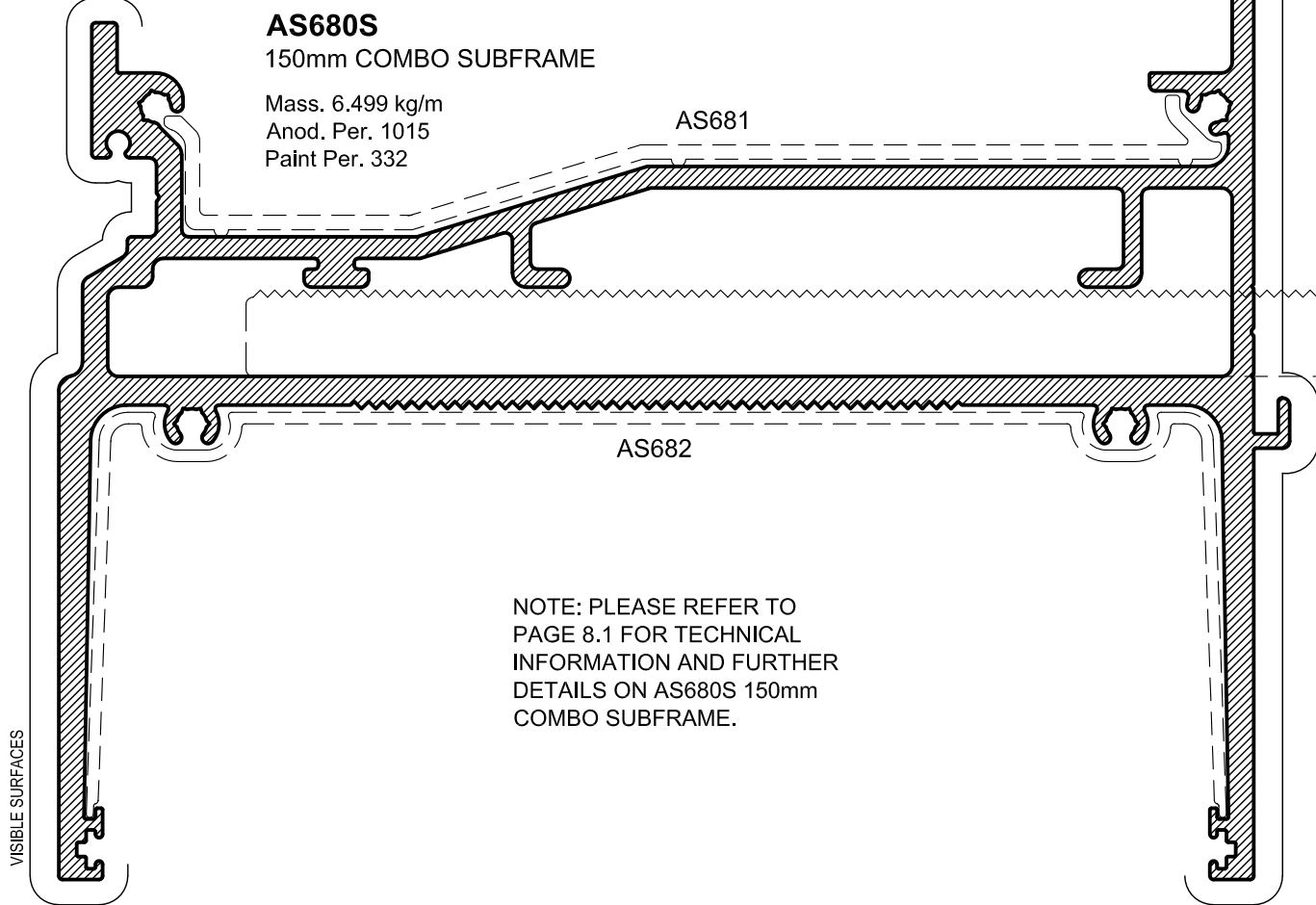
AS682 SUB HEAD SLEEVE Mass. 1.192 kg/m Anod. Per. 553 No Visible Surface
