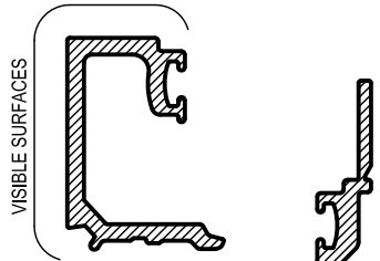
AS659 BEAD (FOR AS660S) Mass. 0.337 kg/m Anod Per. 133 Paint Per. 100
