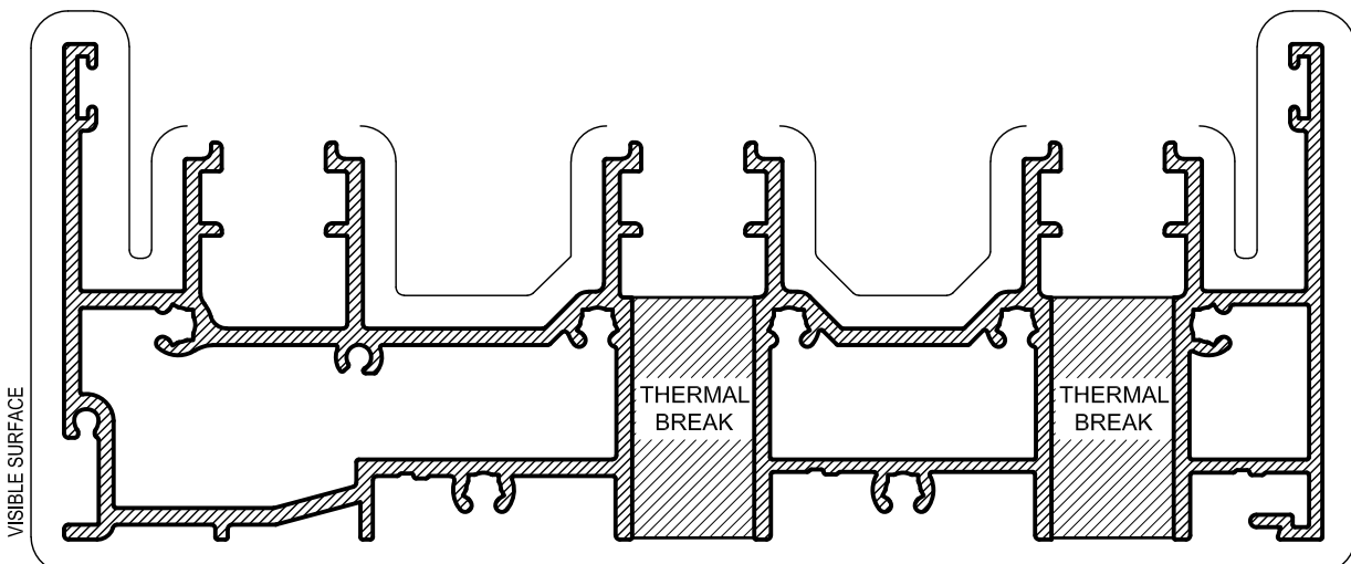
TSD263S 152.4mm SUMP SILL Mass. 3.237 Kg/m Anod. Per. 1111 Paint Per. 417
