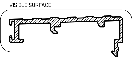
TSD166 STACKER RAMP THRESHOLD Mass. 0.43 Kg/m Anod. Per. 181.6 Paint Per. 100
