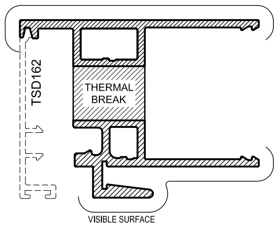
Mass. 1.403 Kg/m Anod. Per. 410 Paint Per. 175 Ixx = 115.1 x 10 3 mm 4
