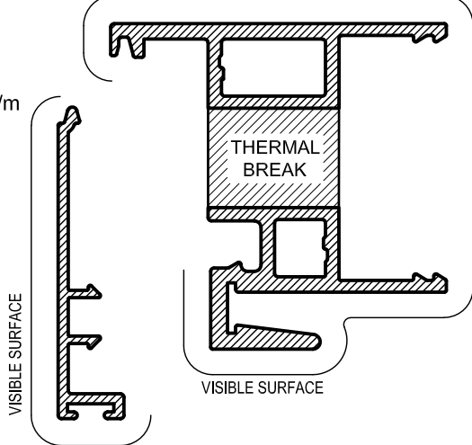
TSD202 STANDARD INTERLOCK Mass. 1.224 Kg/m Anod. Per. 351 Paint Per. 112 Ixx = 105 x 10 3 mm 4
