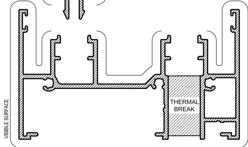
TSD242S 101.6mm SILL Mass. 2.241 Kg/m Anod. Per. 832 Paint Per. 407
