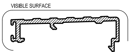
TSD165 RAMP THRESHOLD Mass. 0.4 Kg/m Anod. Per. 172 Paint Per. 100
