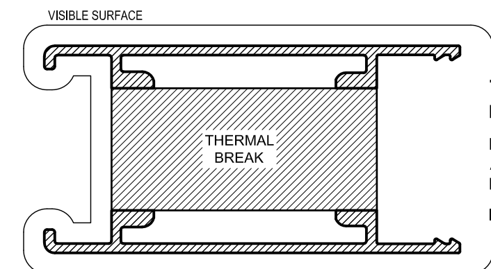
TSD201 LOCK STILE Mass. 1.592 Kg/m Anod. Per. 434 Paint Per. 208 Ixx = 115.6 x 10 3 mm 4
