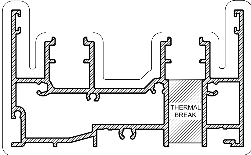
TSD243S 101.6mm SUMP SILL Mass. 2.668 Kg/m Anod. Per. 785 Paint Per. 340
