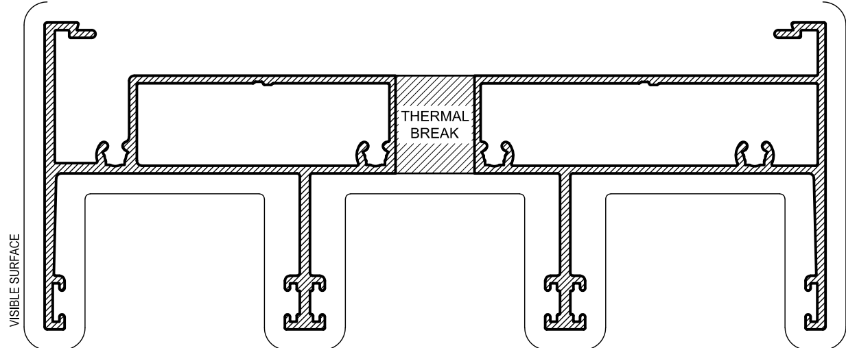
TSD261 152.4mm HEAD Mass. 2.691 Kg/m Anod. Per. 858 Paint Per. 476 Ixx = 2030 x 10 3 mm 4 Iyy = 194.4 x 10 3 mm 4
