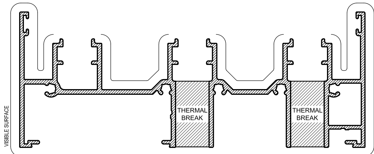
TSD262S 152.4mm SILL Mass. 3.159 Kg/m Anod. Per. 1194 Paint Per. 485
