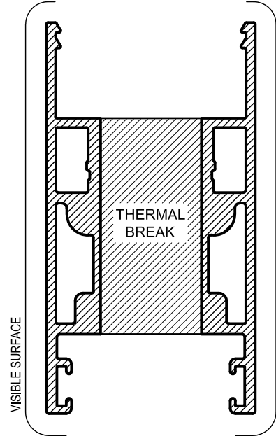
TSD207 DOOR RAIL Mass. 1.622 Kg/m Anod. Per. 456 Paint Per. 160 Ixx = 114.1 x 10 3 mm 4
