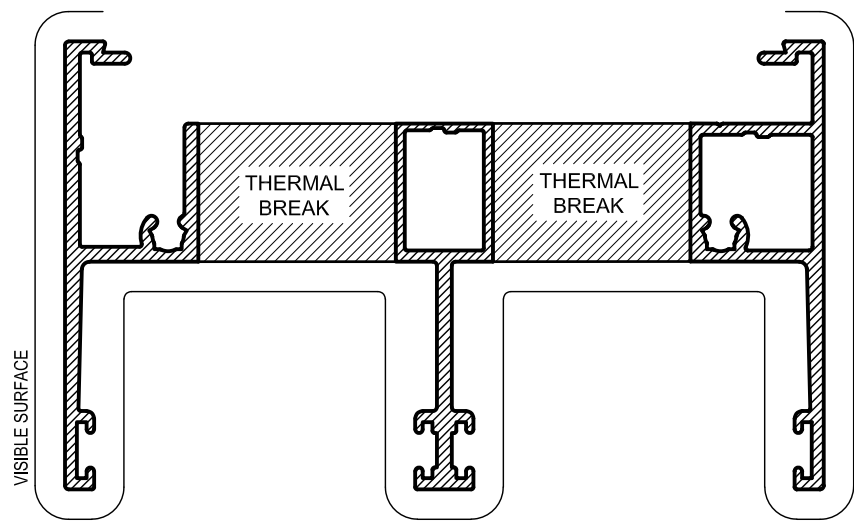
TSD241 101.6mm HEAD Mass. 1.863 Kg/m Anod. Per. 678 Paint Per. 294 Ixx = 681 x 10 3 mm 4 Iyy = 126.7 x 10 3 mm 4
