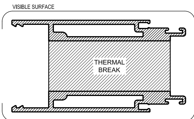
TSD205 MALE MEETING STILE Mass. 1.552 Kg/m Anod. Per. 456 Paint Per. 166 Ixx = 105.7 x 10 3 mm 4
