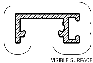
AS9 CONCEALED PLANT ON DOOR STOP Mass. 0,315 Kg/m Anod. Per. 125 Paint Per. 100
