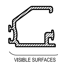
ECO114* 16mm ADAPTOR (SLIDE IN) Mass. 0,259 Kg/m Anod. Per. 136 Paint Per. 100
