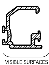
ECO115 20mm ADAPTOR (SLIDE IN) Mass. 0,236 Kg/m Anod. Per. 124 Paint Per. 100
