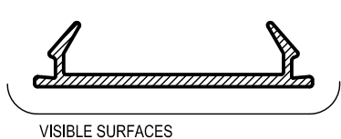
ECO208R FLUSH POCKET INFILL DG Mass. 0,253 Kg/m Anod. Per. 119 Paint Per. 100
