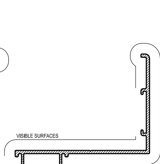
AF45 McARTHUR EVO LOUVRE SILL ADAPTOR Mass. 0.556 Kg/m Anod. Per. 293 Paint Per. 135
