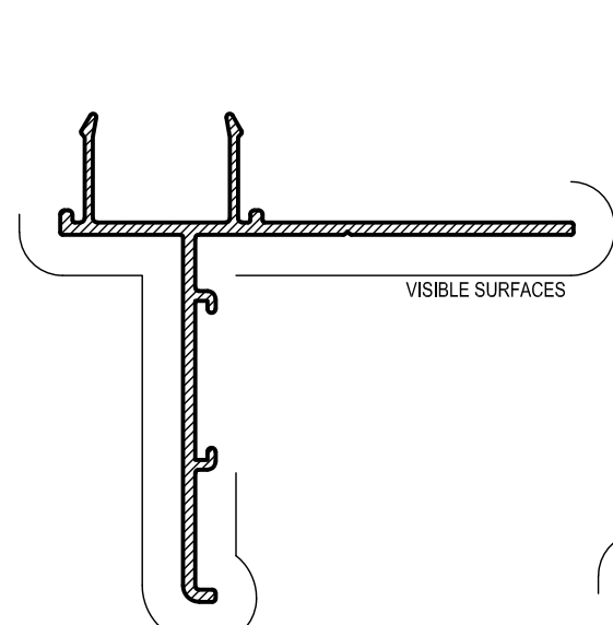
AF44 McARTHUR EVO LOUVRE HEAD ADAPTOR Mass. 0.556 Kg/m Anod. Per. 293 Paint Per. 138
