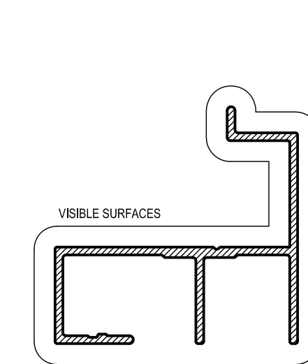
ASW43 AWNING WINDER ADAPTOR Mass. 0.624 Kg/m Anod. Per. 299 Paint Per. 160
