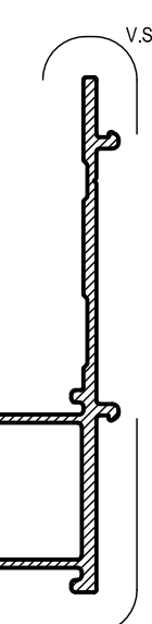
AF43 McARTHUR EVO LOUVRE ADAPTOR Mass. 0.377 Kg/m Anod. Per. 197 Paint Per. 100
