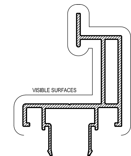
ASW118 McARTHUR EVO PROTILT AWNING ADAPTOR Mass. 0.858 Kg/m Anod. Per. 337 Paint Per. 172
