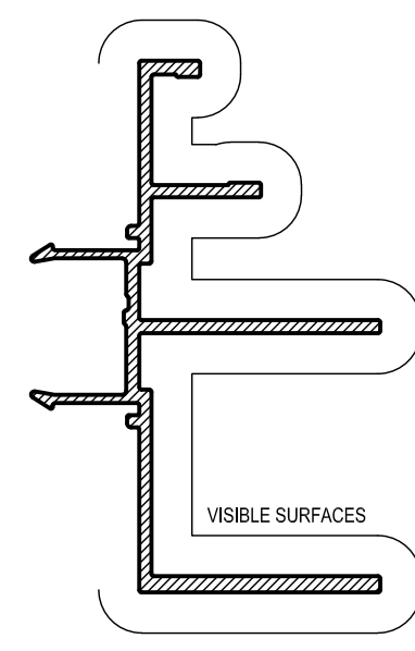
VM75 SASH SCREEN RECEIVER ADAPTOR Mass. 0.734 Kg/m Anod. Per. 346 Paint Per. 225
