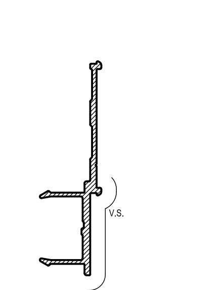
AF54 McARTHUR EVO SLIM LOUVRE ADAPTOR Mass. 0.337 Kg/m Anod. Per. 171 Paint Per. 100
