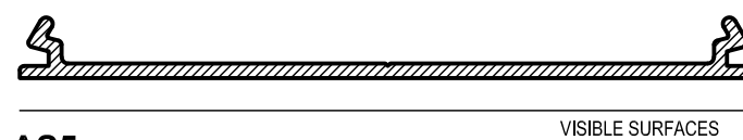
AS5 FLUSH ADAPTOR Mass. 0.500 Kg/m Anod. Per. 213 Paint Per. 100 lxx = 150.5 x 10 3 mm 4
