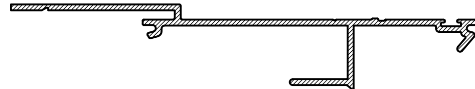
ME19 100mm FIXING LEG ADAPTOR Mass. 0.973 Kg/m Anod. Per. 391 Paint Per. 100
