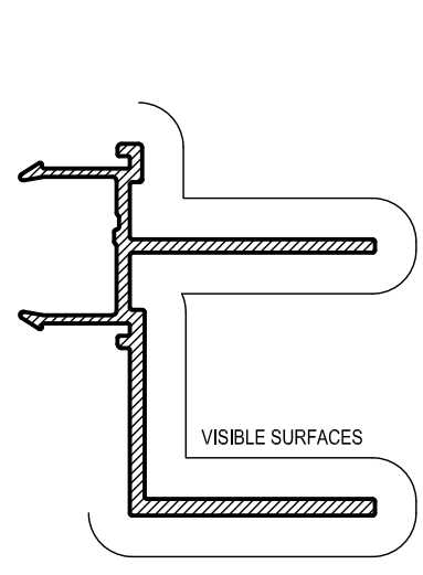
VM76 SASH RECEIVER ADAPTOR Mass. 0.734 Kg/m Anod. Per. 346 Paint Per. 225
