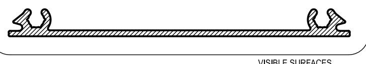
AS5F FLUSH ADAPTOR WITH SCREW FLUTES Mass. 0.538 Kg/m Anod. Per. 231 Paint Per. 100 lxx = 180.0 x 10 3 mm 4
