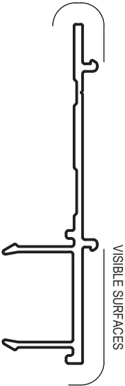
AF43 McARTHUR EVO LOUVRE ADAPTOR Mass. 0.377 Kg/m Anod. Per. 197 Paint Per. 100
