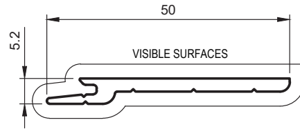
LP1 LOCK PROTECTOR
