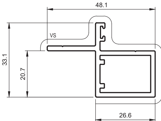
HD12 HD SCREEN ADAPTOR Anod. Per. 164 Paint Per. 123
