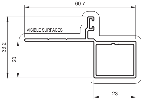
HD16 LONG LEG DOOR REVEAL Anod. Per. 200 Paint Per. 143
