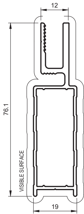
SD50 COMBO DOOR FRAME STD Anod. Per. 263 Paint Per. 206
