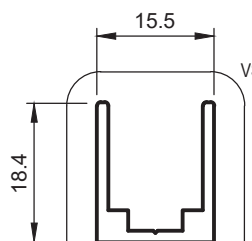
ST007 SECURITY SCREEN TRACK
