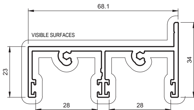
ST20 DOUBLE SCREEN TRACK 28mm HEAD
