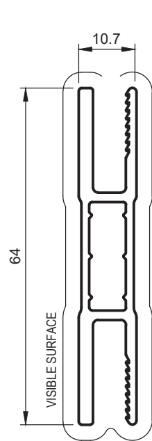
SW63 11mm ALU-GARD EDGE WINDOW FRAME WITH LEG (ALU3) Anod. Per. 182 Paint Per. 129
