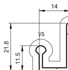
HD1 BOTTOM SILL TRACK
