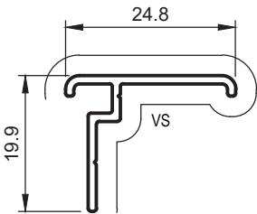
TM18 OFFSET T MULLION Anod. Per. 100 Paint Per. 100
