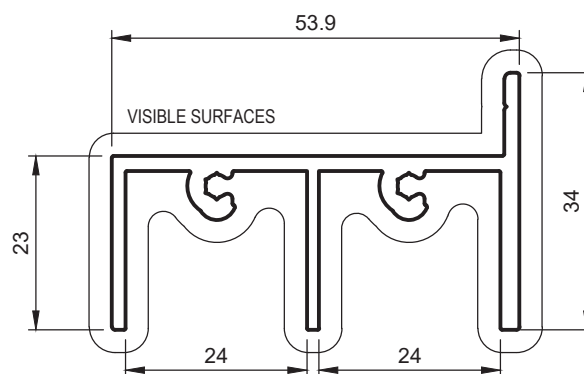
ST23 DOUBLE SCREEN TRACK 24mm HEAD
