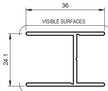
ST15 RECEIVER CHANNEL
