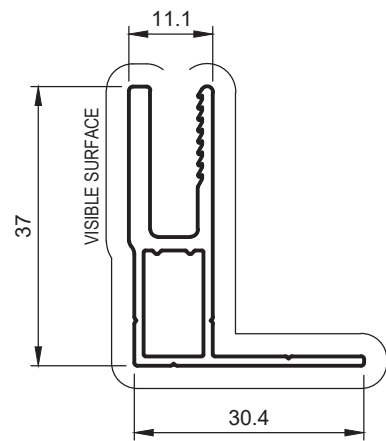
SW63 11mm ALU-GARD EDGE WINDOW FRAME WITH LEG (ALU3) Anod. Per. 182 Paint Per. 129
