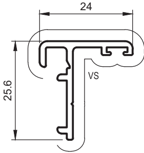
TM5 SECURITY T MULLION Anod. Per. 126 Paint Per. 100
