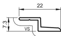
HD10 EXTENDED 7mm OFFSET INTERLOCK
