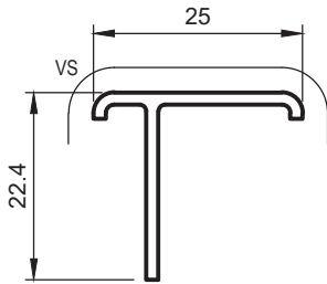
TM4 T MULLION Anod. Per. 100 Paint Per. 100
