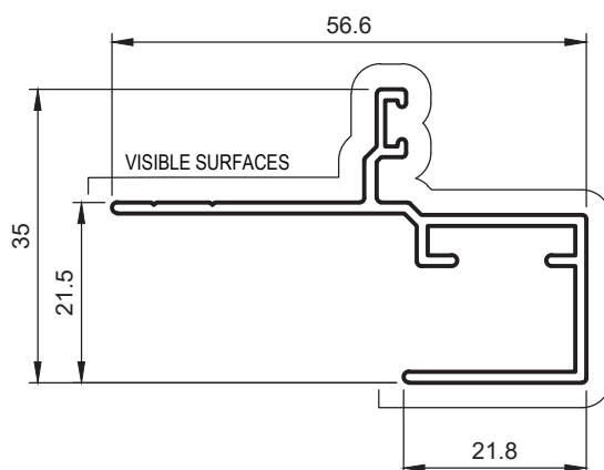
HD20 SECURITY JAMB
