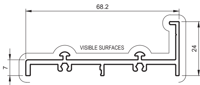
ST21 DOUBLE SCREEN TRACK 28mm SILL
