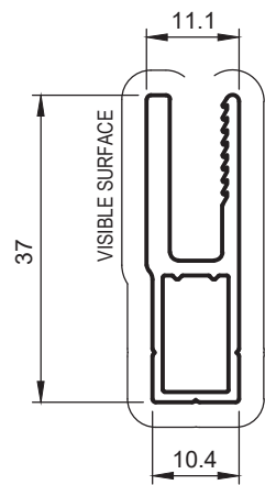
SW62 ALU-GARD EDGE 11mm WINDOW FRAME Anod. Per. 142 Paint Per. 100
