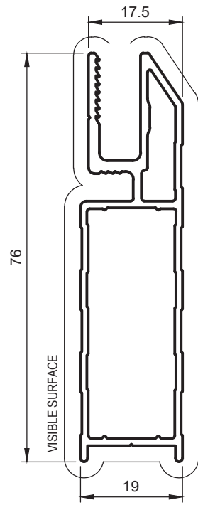
SD51 COMBO DOOR FRAME HD Anod. Per. 255 Paint Per. 253
