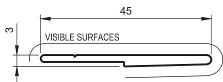
HD21 HEAVY DUTY FLAT INTERLOCK
