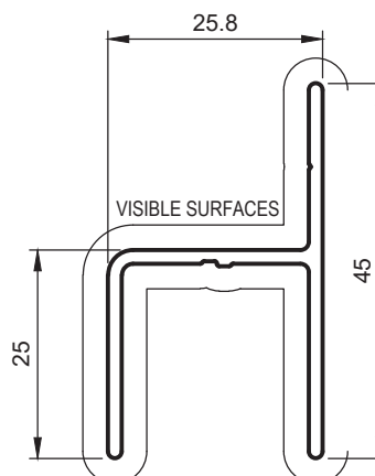
ST16 TOP TRACK FOR SCREEN DOOR
