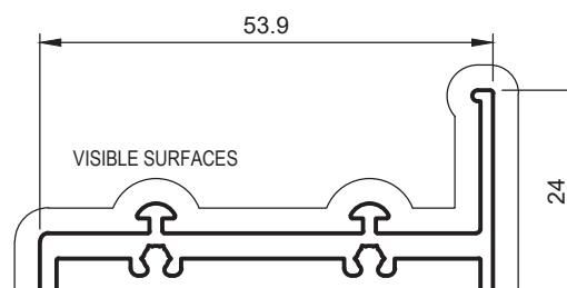
ST24 DOUBLE SCREEN TRACK 24mm SILL
