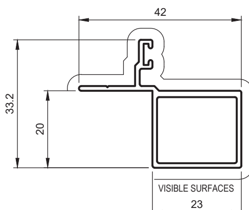
HD15 SHORT LEG DOOR REVEAL
