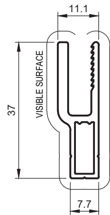
SW61 ALU-GARD EDGE 9mm WINDOW FRAME Anod. Per. 141 Paint Per. 100
