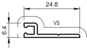
BS2 BUGSTRIP LONG LEG Anod. Per. 100 Paint Per. 100
