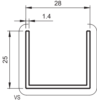
HD19 CHANNEL 28 x 25 x 1.6mm Anod. Per. 153 Paint Per. 100
