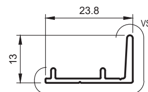
HD29 ALTITUDE / CARINYA INTERLOCK
