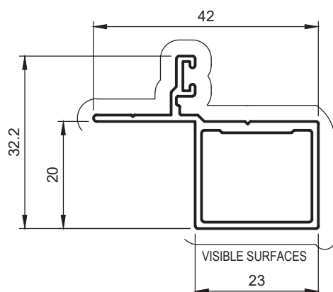
HD27 SHORT LEG DOOR REVEAL
