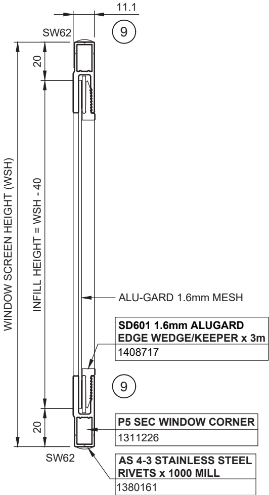
SW62 11mm FRAME
