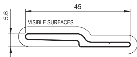
HD22 HEAVY DUTY STEPPED INTERLOCK
