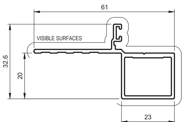
HD26 LONG LEG DOOR REVEAL
