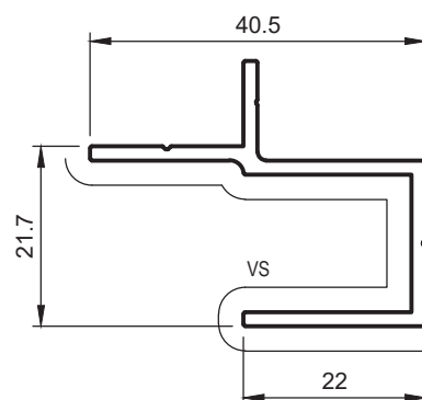
HD11 SECURITY JAMB
