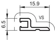
BS1 BUGSTRIP SHORT LEG Anod. Per. 100 Paint Per. 100
