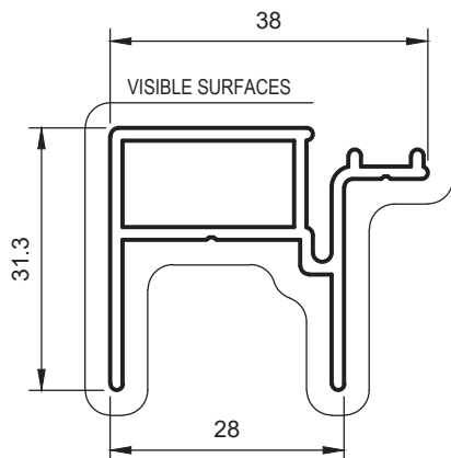
ST10 RECEIVER JAMB
