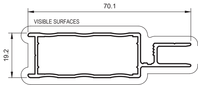
SD3 DOOR FRAME Anod. Per. 229 Paint Per. 193
