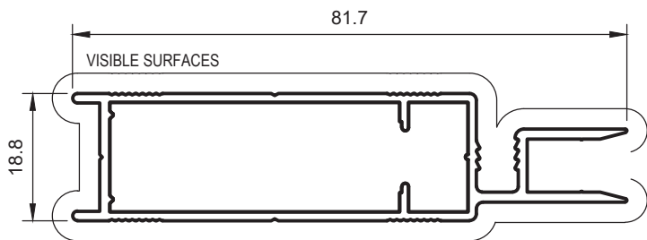
SD14 DOOR FRAME Anod. Per. 258 Paint Per. 176
