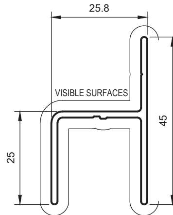
ST16 TOP TRACK FOR SCREEN DOOR
