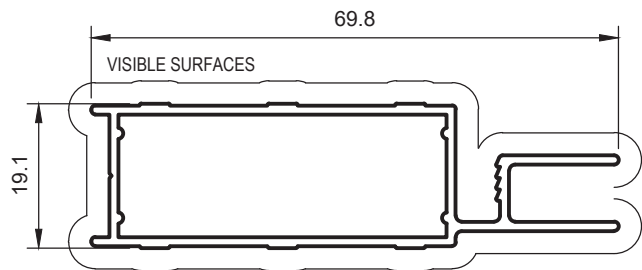
SD7 DOOR FRAME Anod. Per. 229 Paint Per. 194
