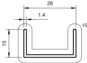
HD17 CHANNEL 28 x 15 x 1.4mm Anod. Per. 112 Paint Per. 112
