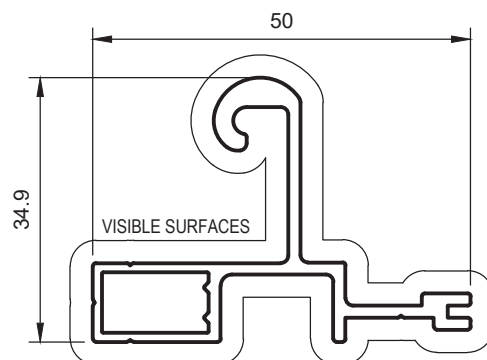
SW25 OUTWARD OPENING STD HINGE PERIMETER FRAME
