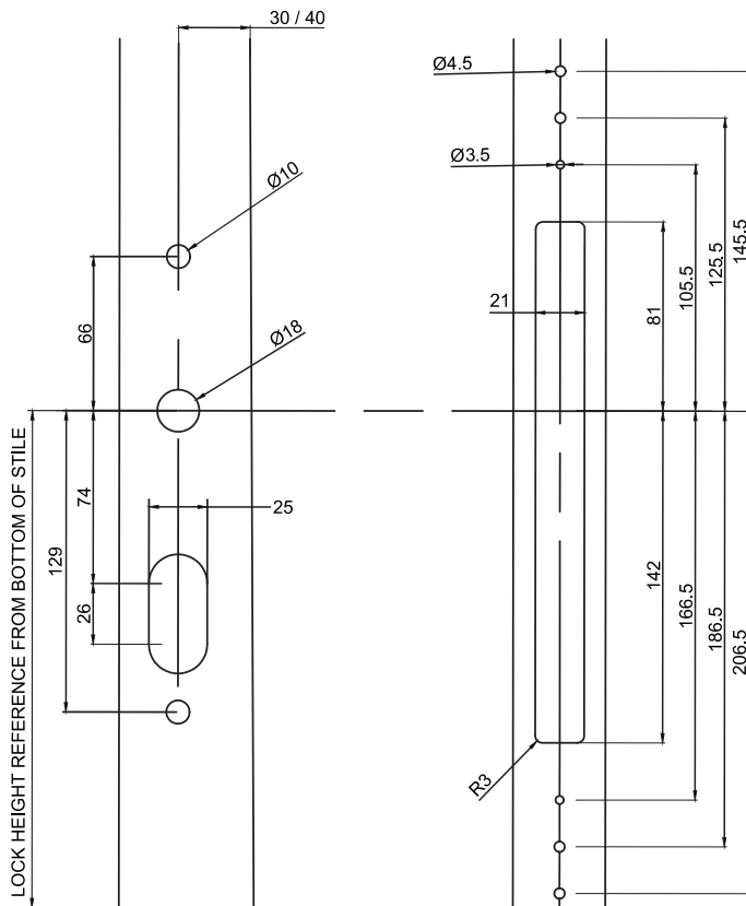
Surface Mounted
